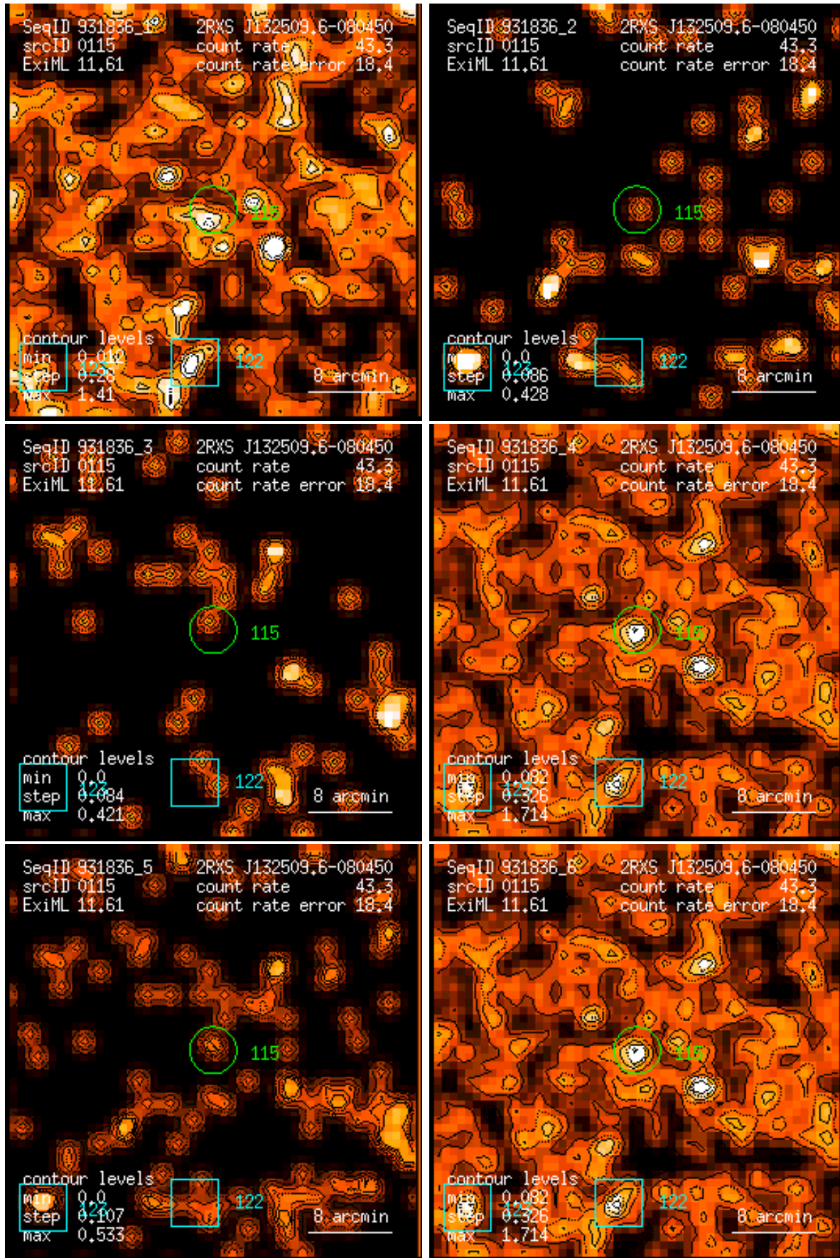
Figure 115: RASS 931836: detection 0115: band rate images, Gaussian filter: (1) PSPC channels 11 – 41, (2) 52 – 90, (3) 91 – 201, (4) 11 – 235, (5) 52 – 201, (6) 11 – 201. Broad band rates in counts/ks. Band rate contour levels in counts/ks/arcmin 2 .
