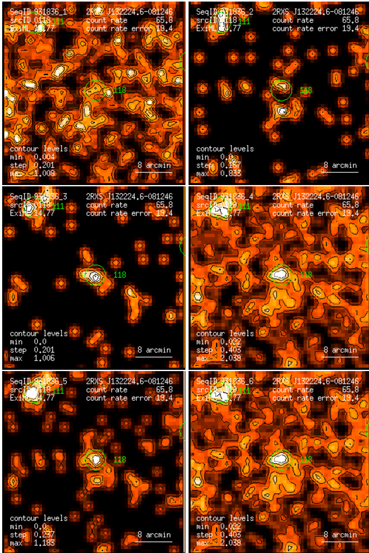
Figure 118: RASS 931836: detection 0118: band rate images, Gaussian filter: (1) PSPC channels 11 – 41, (2) 52 – 90, (3) 91 – 201, (4) 11 – 235, (5) 52 – 201, (6) 11 – 201. Broad band rates in counts/ks. Band rate contour levels in counts/ks/arcmin 2 .
