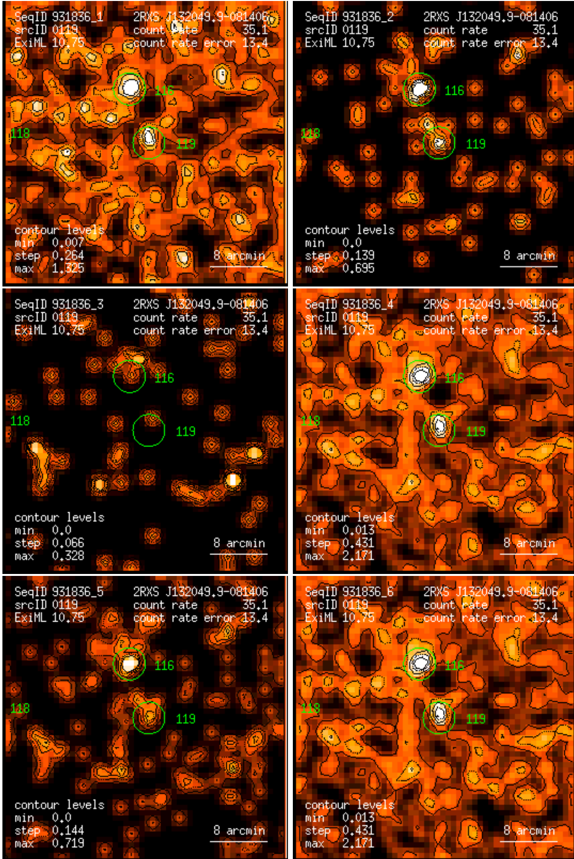
Figure 119: RASS 931836: detection 0119: band rate images, Gaussian filter: (1) PSPC channels 11 – 41, (2) 52 – 90, (3) 91 – 201, (4) 11 – 235, (5) 52 – 201, (6) 11 – 201. Broad band rates in counts/ks. Band rate contour levels in counts/ks/arcmin 2 .
