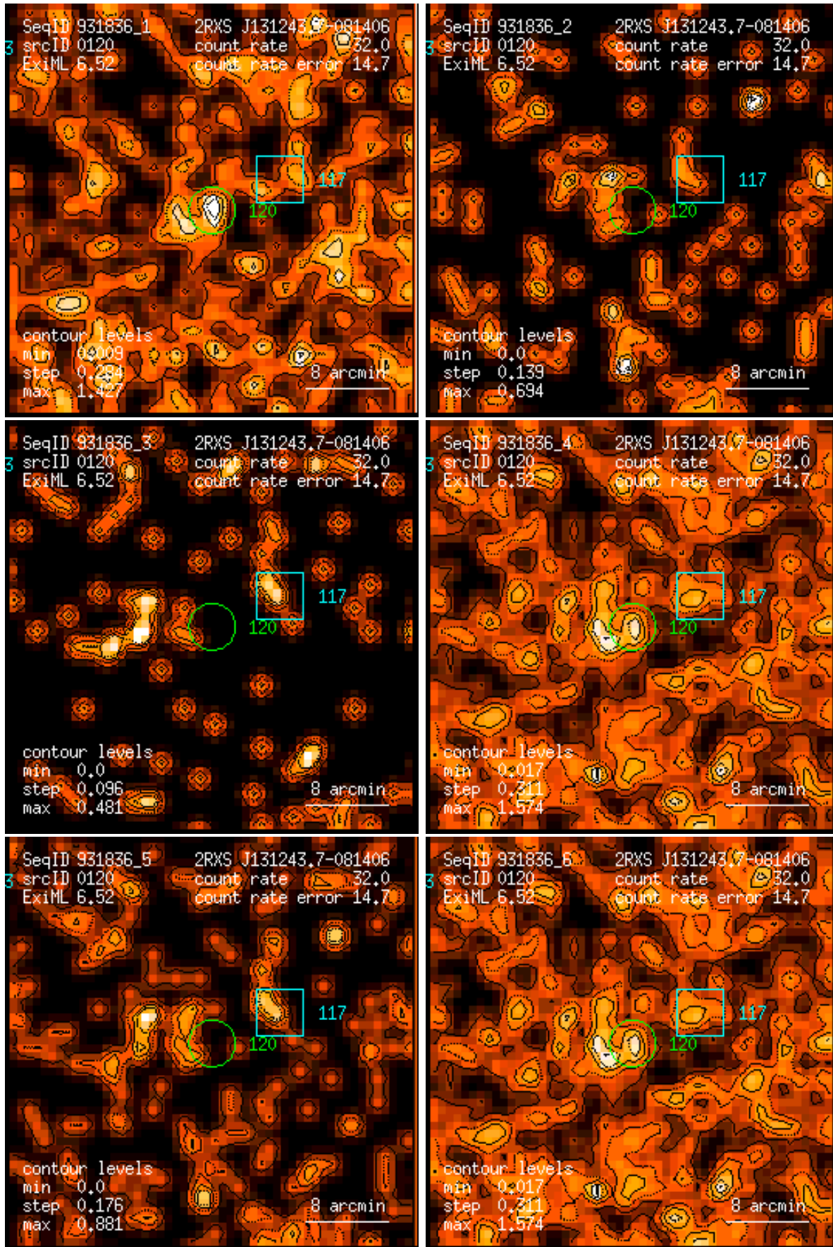
Figure 120: RASS 931836: detection 0120: band rate images, Gaussian filter: (1) PSPC channels 11 – 41, (2) 52 – 90, (3) 91 – 201, (4) 11 – 235, (5) 52 – 201, (6) 11 – 201. Broad band rates in counts/ks. Band rate contour levels in counts/ks/arcmin 2 .
