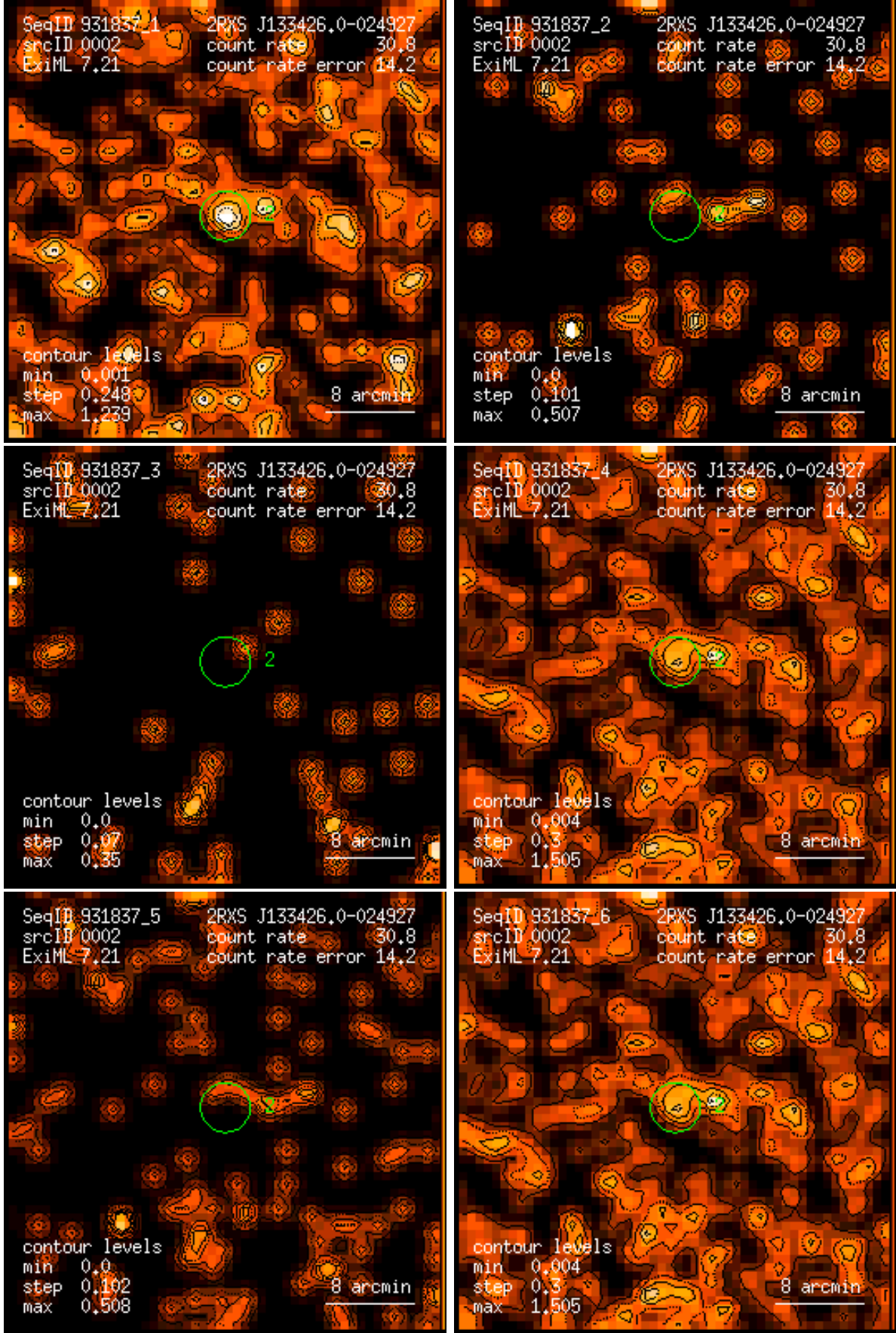
Figure 2: RASS 931837: detection 0002: band rate images, Gaussian filter: (1) PSPC channels 11 – 41, (2) 52 – 90, (3) 91 – 201, (4) 11 – 235, (5) 52 – 201, (6) 11 – 201. Broad band rates in counts/ks. Band rate contour levels in counts/ks/arcmin 2 .
