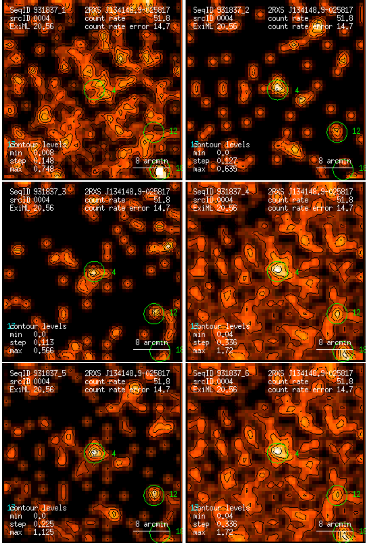
Figure 4: RASS 931837: detection 0004: band rate images, Gaussian filter: (1) PSPC channels 11 – 41, (2) 52 – 90, (3) 91 – 201, (4) 11 – 235, (5) 52 – 201, (6) 11 – 201. Broad band rates in counts/ks. Band rate contour levels in counts/ks/arcmin 2 .
