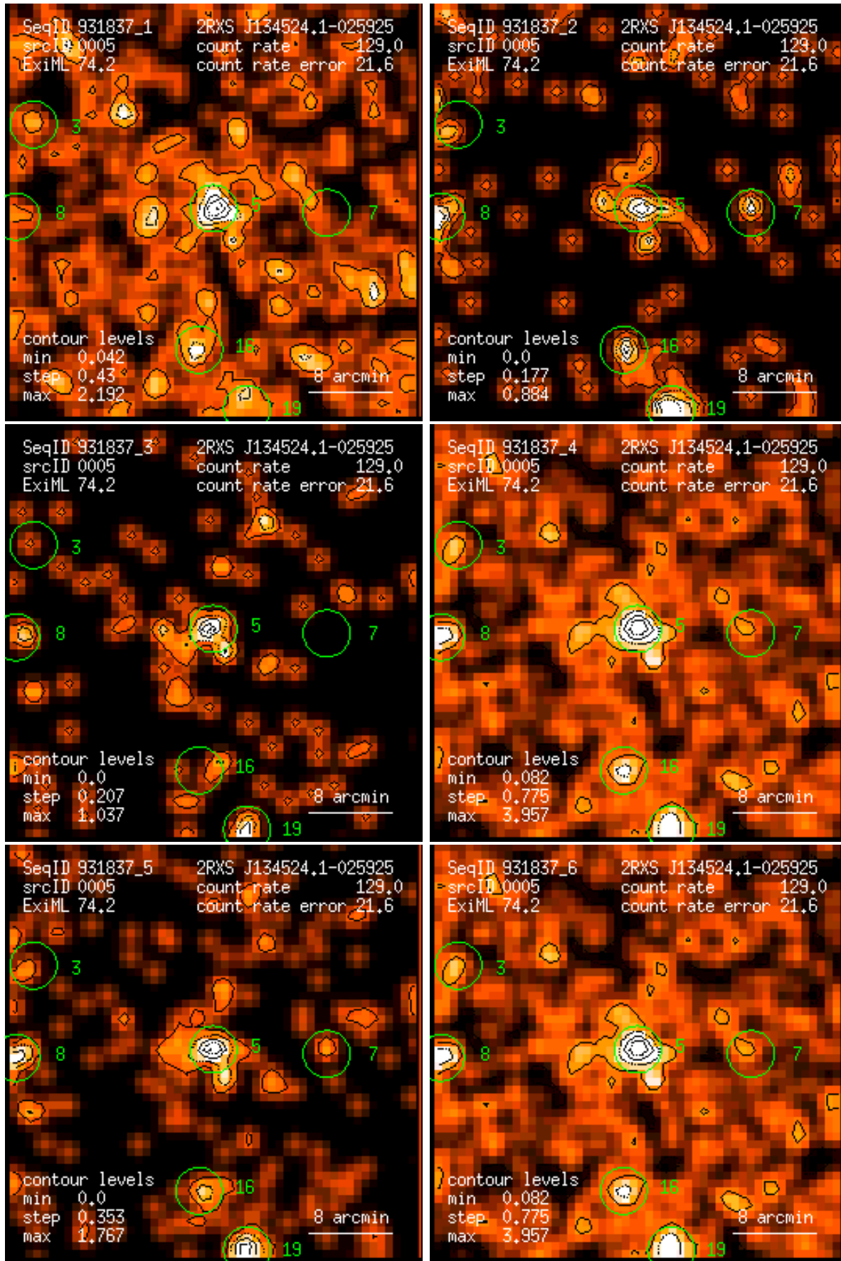
Figure 5: RASS 931837: detection 0005: band rate images, Gaussian filter: (1) PSPC channels 11 – 41, (2) 52 – 90, (3) 91 – 201, (4) 11 – 235, (5) 52 – 201, (6) 11 – 201. Broad band rates in counts/ks. Band rate contour levels in counts/ks/arcmin 2 .
