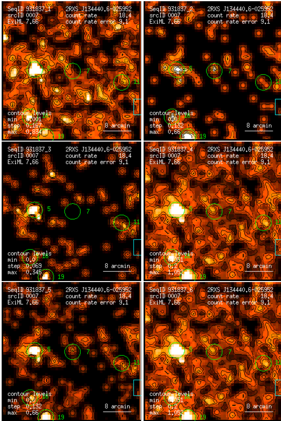
Figure 7: RASS 931837: detection 0007: band rate images, Gaussian filter: (1) PSPC channels 11 – 41, (2) 52 – 90, (3) 91 – 201, (4) 11 – 235, (5) 52 – 201, (6) 11 – 201. Broad band rates in counts/ks. Band rate contour levels in counts/ks/arcmin 2 .
