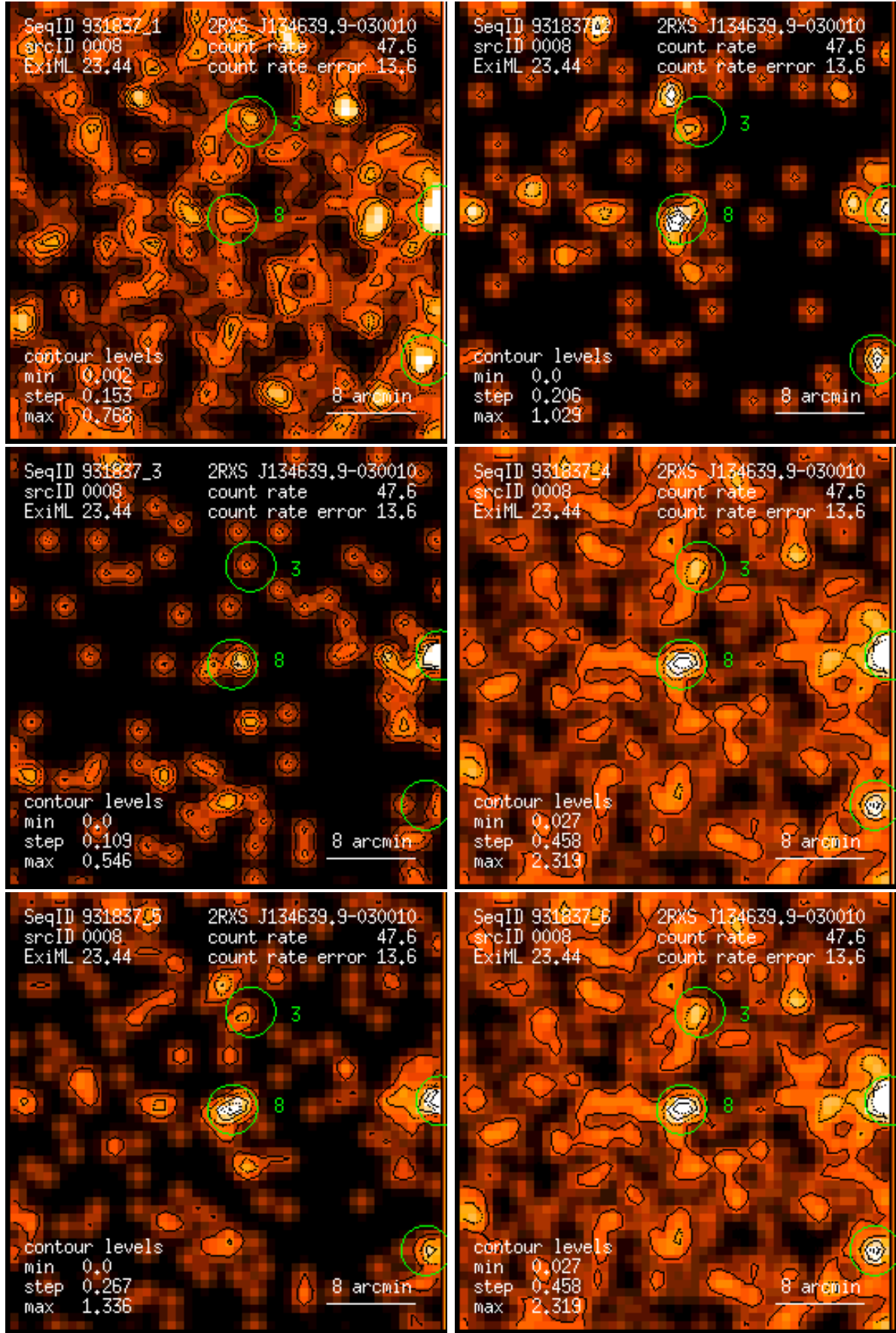
Figure 8: RASS 931837: detection 0008: band rate images, Gaussian filter: (1) PSPC channels 11 – 41, (2) 52 – 90, (3) 91 – 201, (4) 11 – 235, (5) 52 – 201, (6) 11 – 201. Broad band rates in counts/ks. Band rate contour levels in counts/ks/arcmin 2 .
