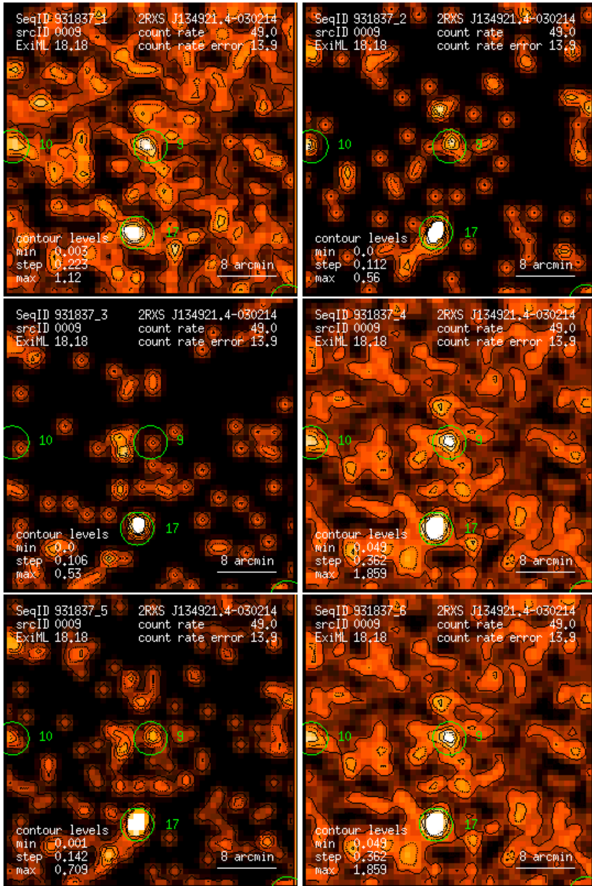
Figure 9: RASS 931837: detection 0009: band rate images, Gaussian filter: (1) PSPC channels 11 – 41, (2) 52 – 90, (3) 91 – 201, (4) 11 – 235, (5) 52 – 201, (6) 11 – 201. Broad band rates in counts/ks. Band rate contour levels in counts/ks/arcmin 2 .
