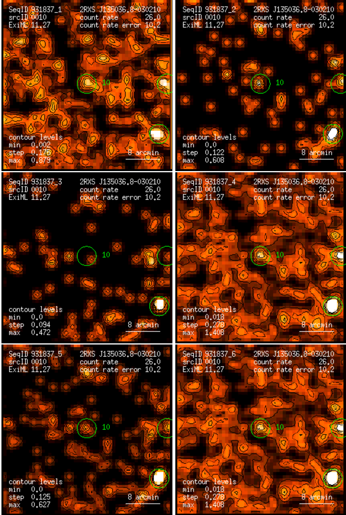
Figure 10: RASS 931837: detection 0010: band rate images, Gaussian filter: (1) PSPC channels 11 – 41, (2) 52 – 90, (3) 91 – 201, (4) 11 – 235, (5) 52 – 201, (6) 11 – 201. Broad band rates in counts/ks. Band rate contour levels in counts/ks/arcmin 2 .
