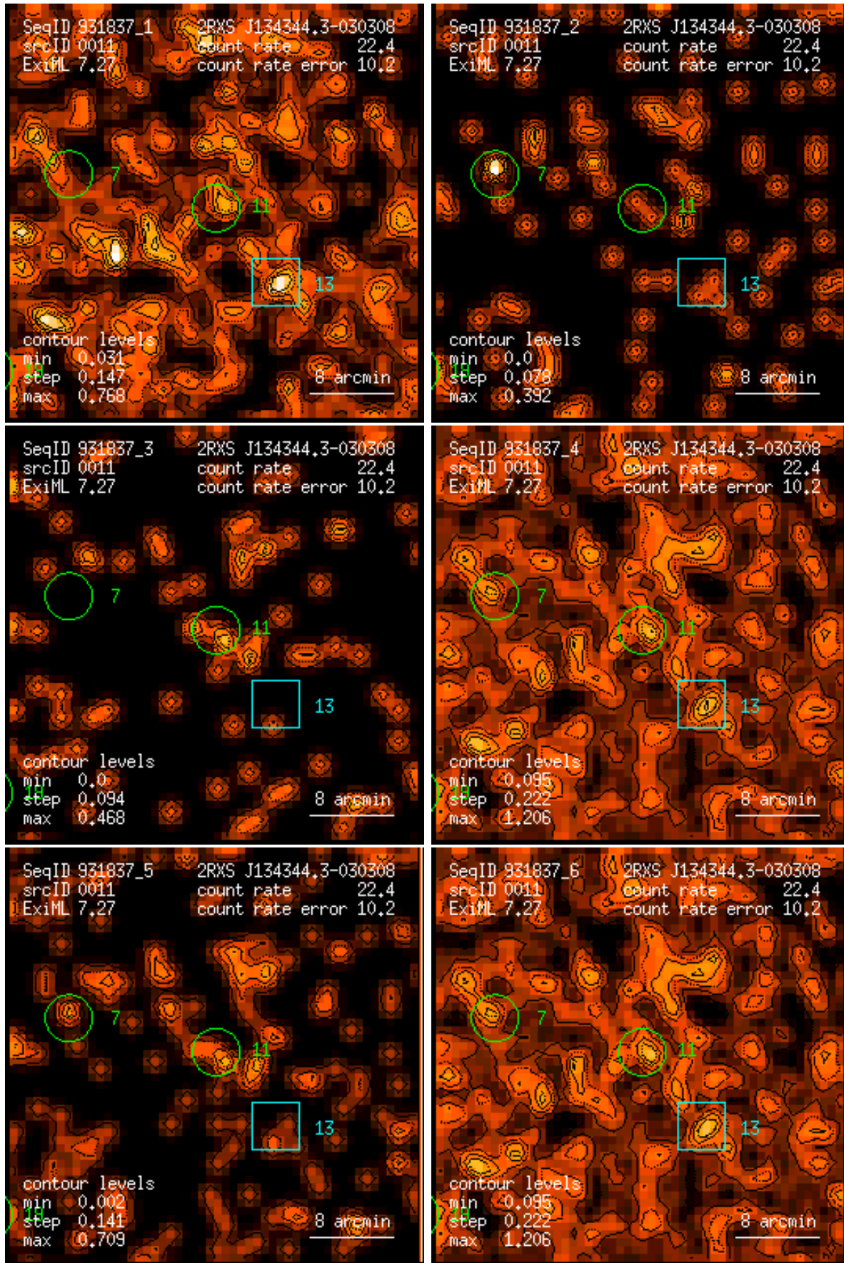
Figure 11: RASS 931837: detection 0011: band rate images, Gaussian filter: (1) PSPC channels 11 – 41, (2) 52 – 90, (3) 91 – 201, (4) 11 – 235, (5) 52 – 201, (6) 11 – 201. Broad band rates in counts/ks. Band rate contour levels in counts/ks/arcmin 2 .
