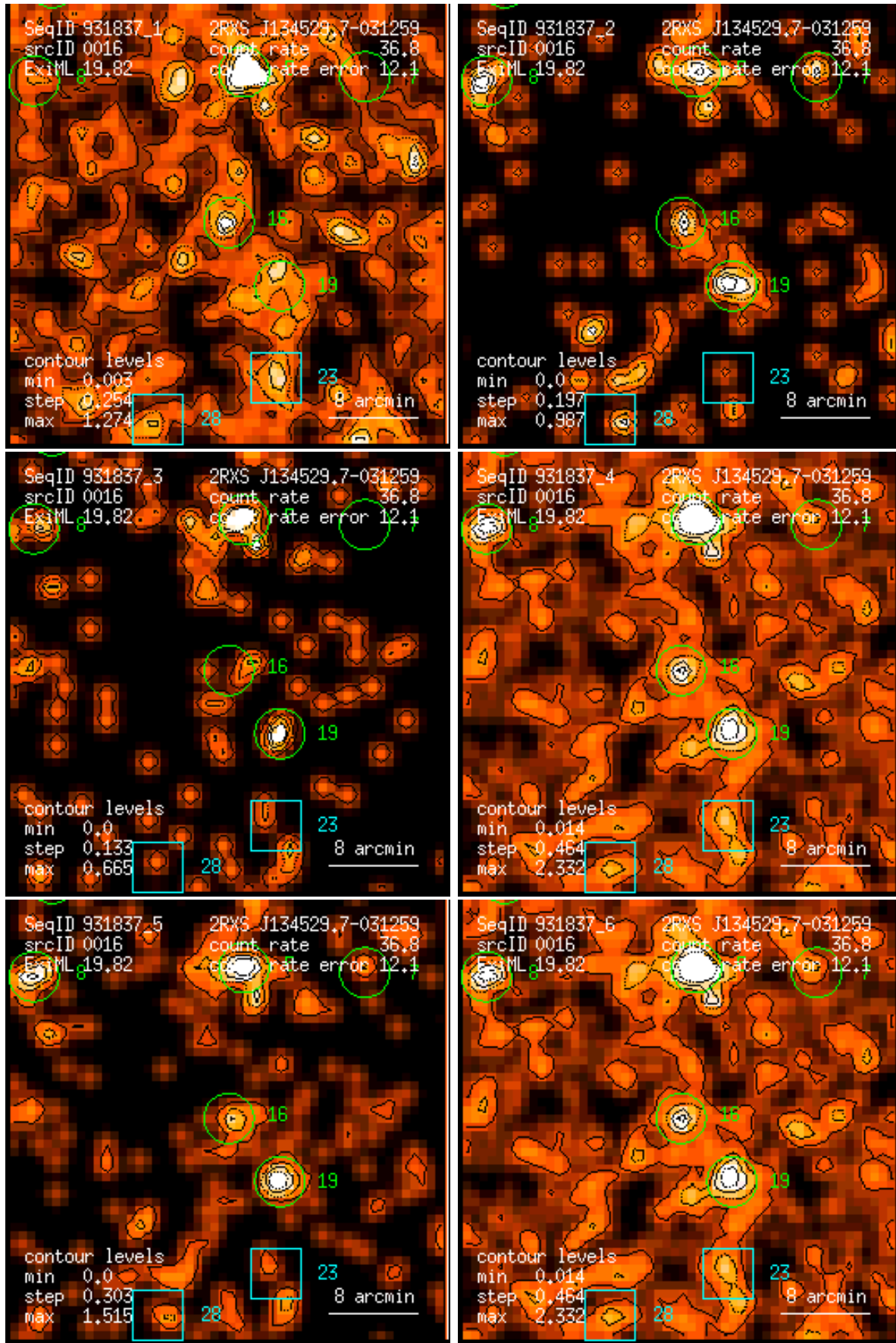
Figure 16: RASS 931837: detection 0016: band rate images, Gaussian filter: (1) PSPC channels 11 – 41, (2) 52 – 90, (3) 91 – 201, (4) 11 – 235, (5) 52 – 201, (6) 11 – 201. Broad band rates in counts/ks. Band rate contour levels in counts/ks/arcmin 2 .
