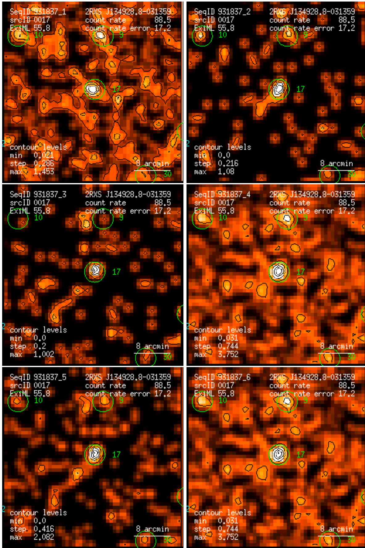
Figure 17: RASS 931837: detection 0017: band rate images, Gaussian filter: (1) PSPC channels 11 – 41, (2) 52 – 90, (3) 91 – 201, (4) 11 – 235, (5) 52 – 201, (6) 11 – 201. Broad band rates in counts/ks. Band rate contour levels in counts/ks/arcmin 2 .
