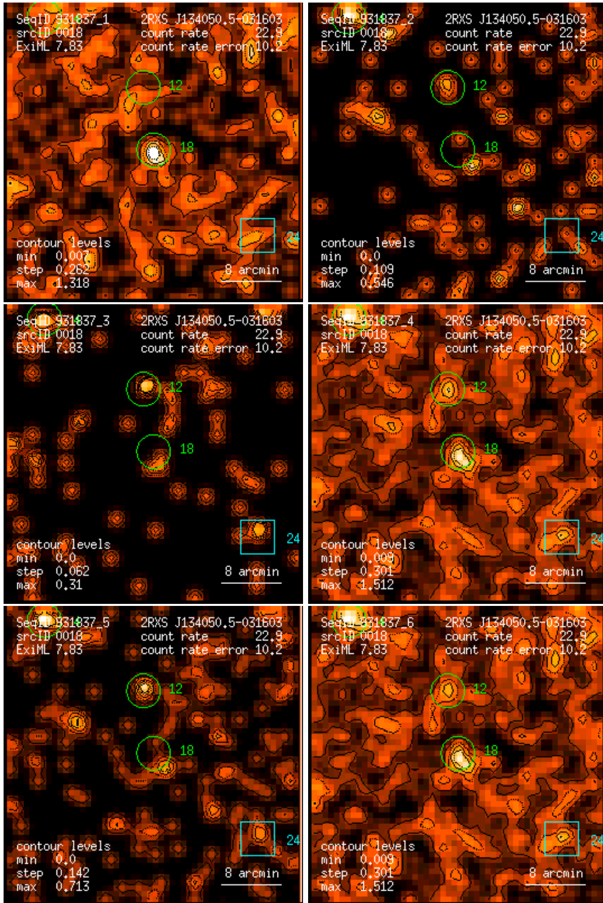
Figure 18: RASS 931837: detection 0018: band rate images, Gaussian filter: (1) PSPC channels 11 – 41, (2) 52 – 90, (3) 91 – 201, (4) 11 – 235, (5) 52 – 201, (6) 11 – 201. Broad band rates in counts/ks. Band rate contour levels in counts/ks/arcmin 2 .
