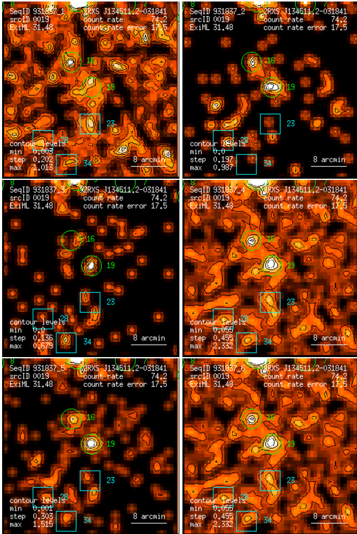
Figure 19: RASS 931837: detection 0019: band rate images, Gaussian filter: (1) PSPC channels 11 – 41, (2) 52 – 90, (3) 91 – 201, (4) 11 – 235, (5) 52 – 201, (6) 11 – 201. Broad band rates in counts/ks. Band rate contour levels in counts/ks/arcmin 2 .
