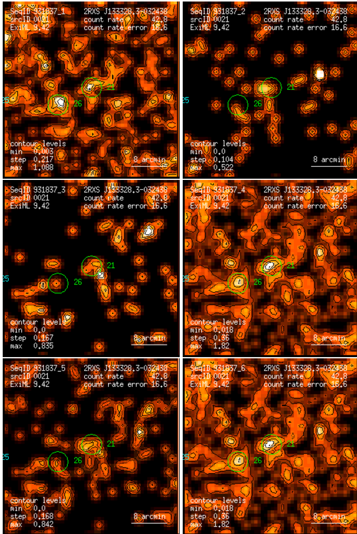
Figure 21: RASS 931837: detection 0021: band rate images, Gaussian filter: (1) PSPC channels 11 – 41, (2) 52 – 90, (3) 91 – 201, (4) 11 – 235, (5) 52 – 201, (6) 11 – 201. Broad band rates in counts/ks. Band rate contour levels in counts/ks/arcmin 2 .
