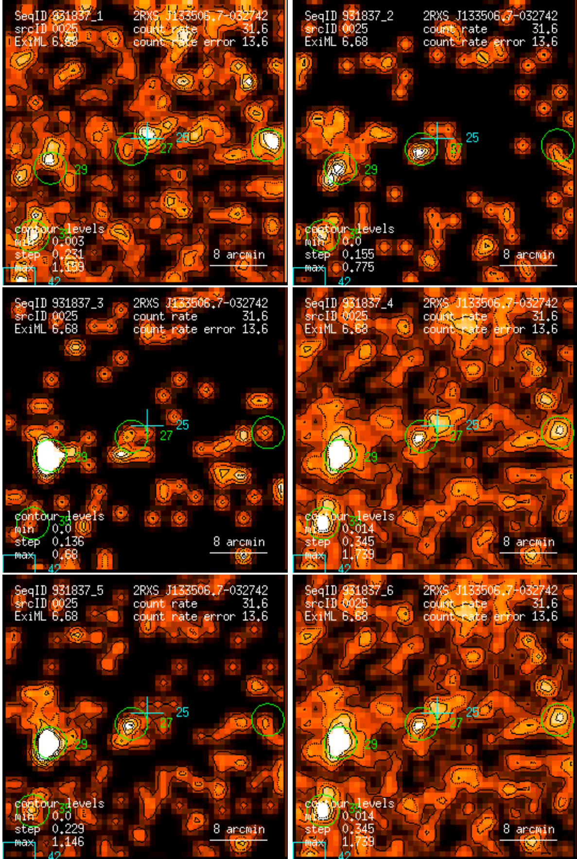
Figure 25: RASS 931837: detection 0025: band rate images, Gaussian filter: (1) PSPC channels 11 – 41, (2) 52 – 90, (3) 91 – 201, (4) 11 – 235, (5) 52 – 201, (6) 11 – 201. Broad band rates in counts/ks. Band rate contour levels in counts/ks/arcmin 2 .
