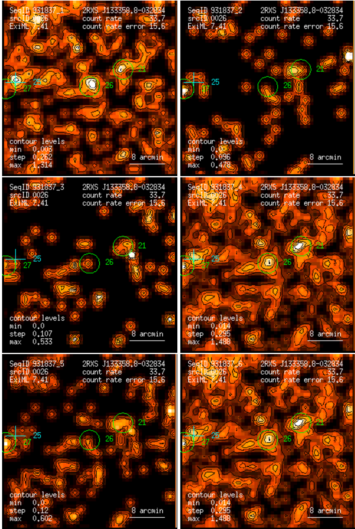
Figure 26: RASS 931837: detection 0026: band rate images, Gaussian filter: (1) PSPC channels 11 – 41, (2) 52 – 90, (3) 91 – 201, (4) 11 – 235, (5) 52 – 201, (6) 11 – 201. Broad band rates in counts/ks. Band rate contour levels in counts/ks/arcmin 2 .
