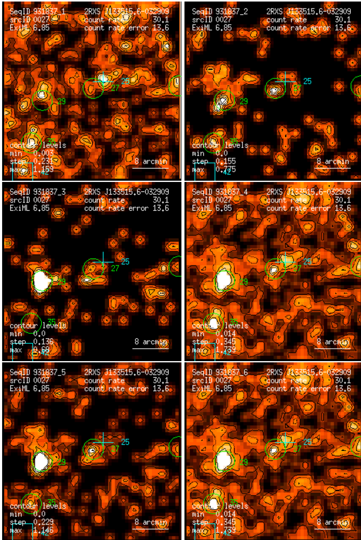
Figure 27: RASS 931837: detection 0027: band rate images, Gaussian filter: (1) PSPC channels 11 – 41, (2) 52 – 90, (3) 91 – 201, (4) 11 – 235, (5) 52 – 201, (6) 11 – 201. Broad band rates in counts/ks. Band rate contour levels in counts/ks/arcmin 2 .
