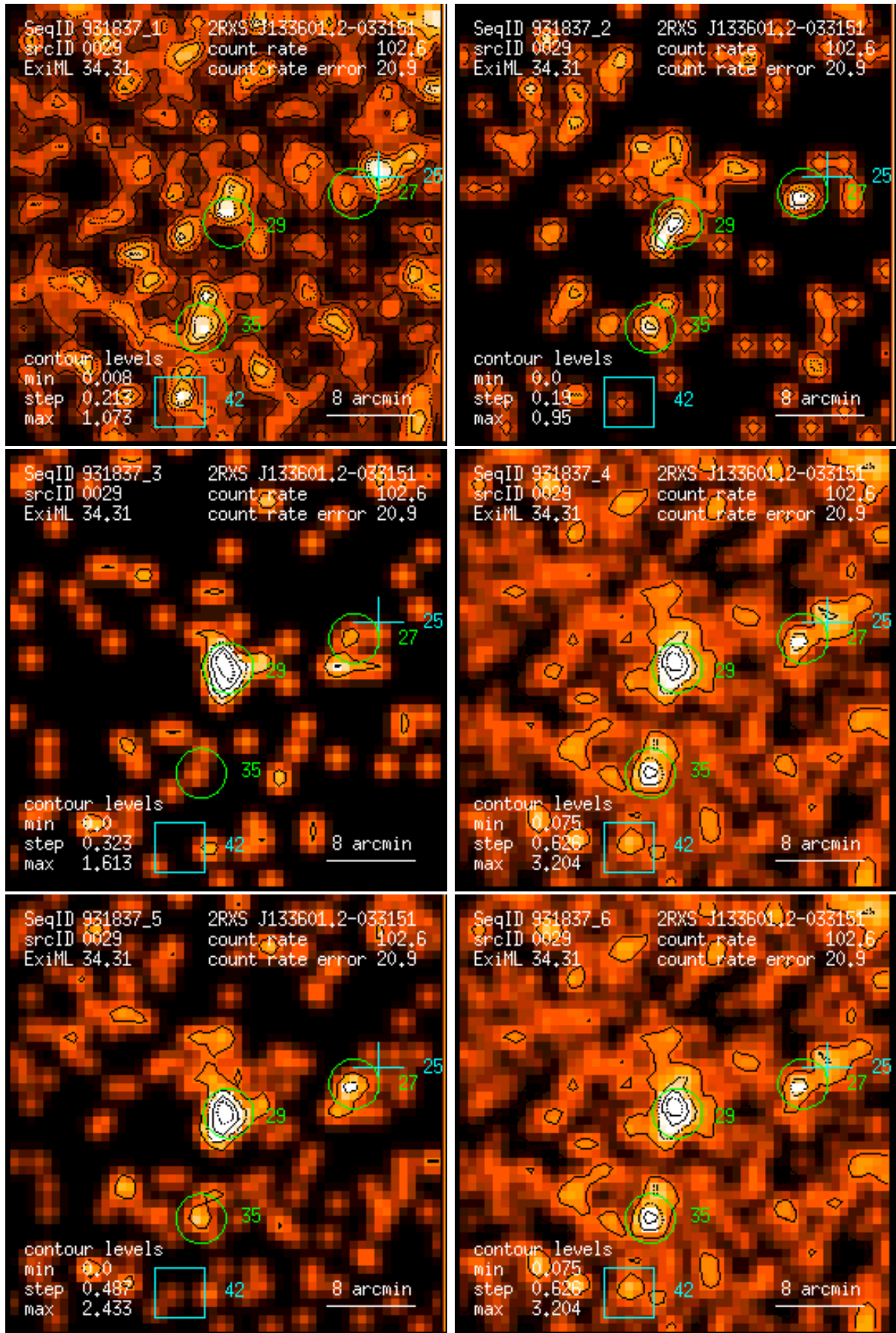
Figure 29: RASS 931837: detection 0029: band rate images, Gaussian filter: (1) PSPC channels 11 – 41, (2) 52 – 90, (3) 91 – 201, (4) 11 – 235, (5) 52 – 201, (6) 11 – 201. Broad band rates in counts/ks. Band rate contour levels in counts/ks/arcmin 2 .
