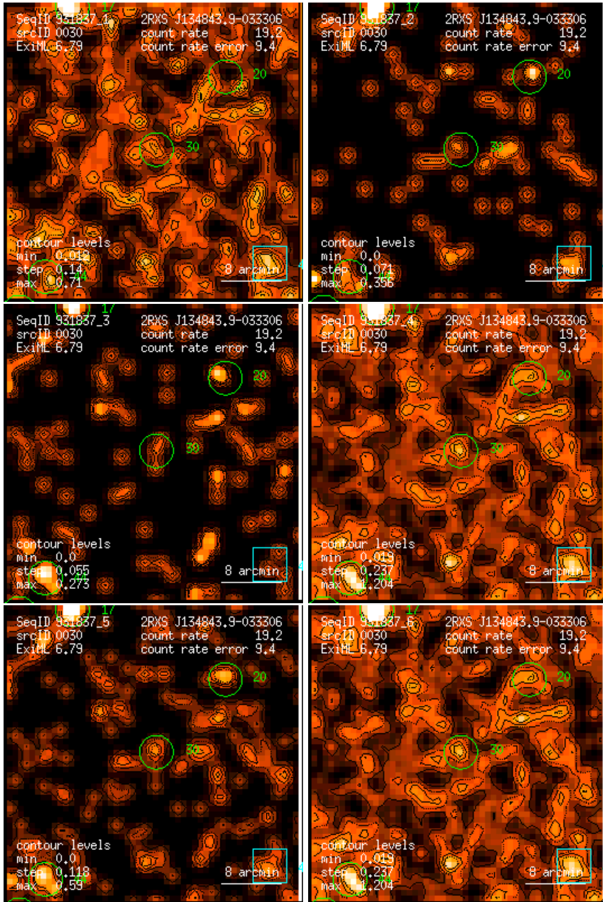
Figure 30: RASS 931837: detection 0030: band rate images, Gaussian filter: (1) PSPC channels 11 – 41, (2) 52 – 90, (3) 91 – 201, (4) 11 – 235, (5) 52 – 201, (6) 11 – 201. Broad band rates in counts/ks. Band rate contour levels in counts/ks/arcmin 2 .
