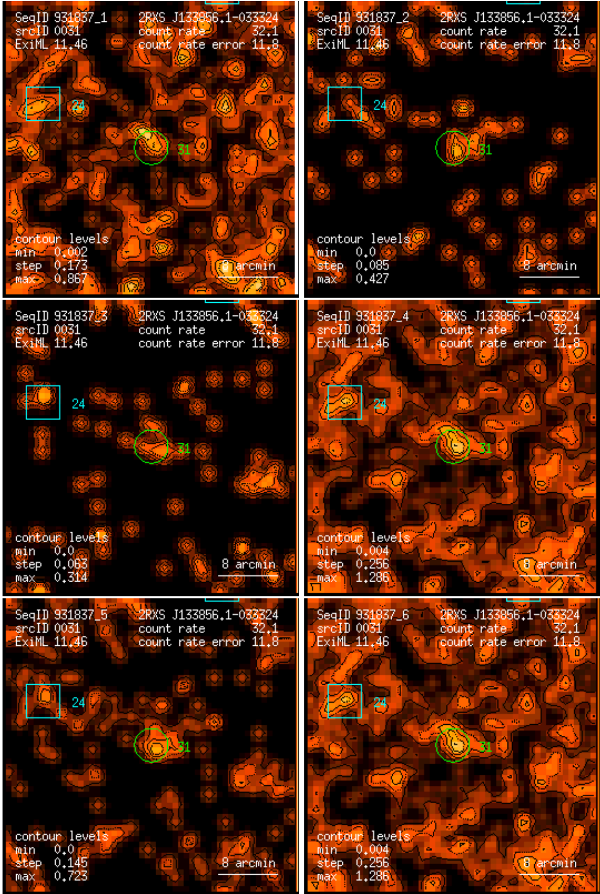
Figure 31: RASS 931837: detection 0031: band rate images, Gaussian filter: (1) PSPC channels 11 – 41, (2) 52 – 90, (3) 91 – 201, (4) 11 – 235, (5) 52 – 201, (6) 11 – 201. Broad band rates in counts/ks. Band rate contour levels in counts/ks/arcmin 2 .
