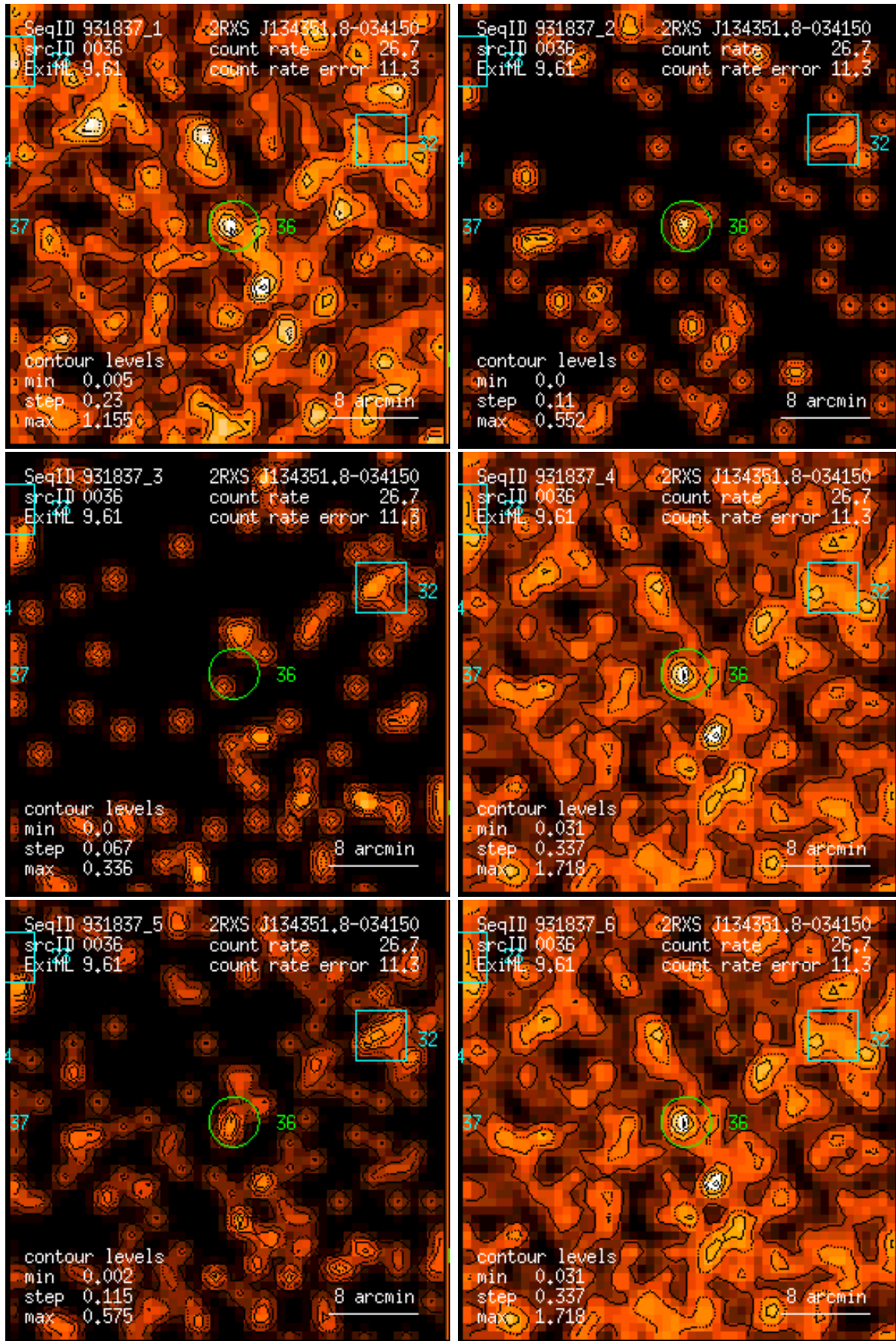
Figure 36: RASS 931837: detection 0036: band rate images, Gaussian filter: (1) PSPC channels 11 – 41, (2) 52 – 90, (3) 91 – 201, (4) 11 – 235, (5) 52 – 201, (6) 11 – 201. Broad band rates in counts/ks. Band rate contour levels in counts/ks/arcmin 2 .
