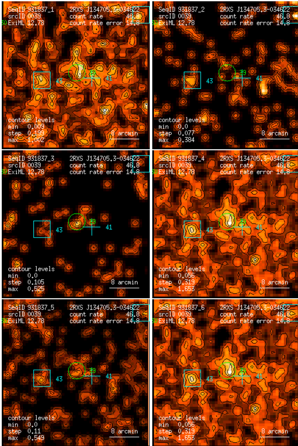
Figure 39: RASS 931837: detection 0039: band rate images, Gaussian filter: (1) PSPC channels 11 – 41, (2) 52 – 90, (3) 91 – 201, (4) 11 – 235, (5) 52 – 201, (6) 11 – 201. Broad band rates in counts/ks. Band rate contour levels in counts/ks/arcmin 2 .
