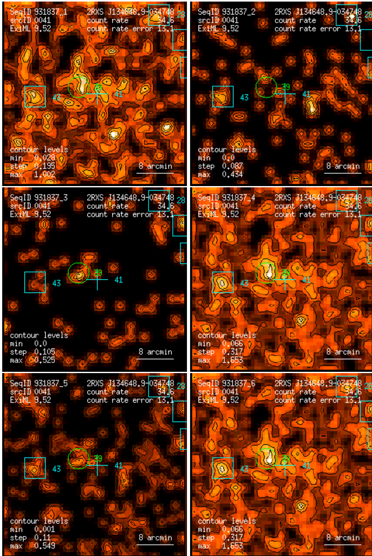
Figure 41: RASS 931837: detection 0041: band rate images, Gaussian filter: (1) PSPC channels 11 – 41, (2) 52 – 90, (3) 91 – 201, (4) 11 – 235, (5) 52 – 201, (6) 11 – 201. Broad band rates in counts/ks. Band rate contour levels in counts/ks/arcmin 2 .
