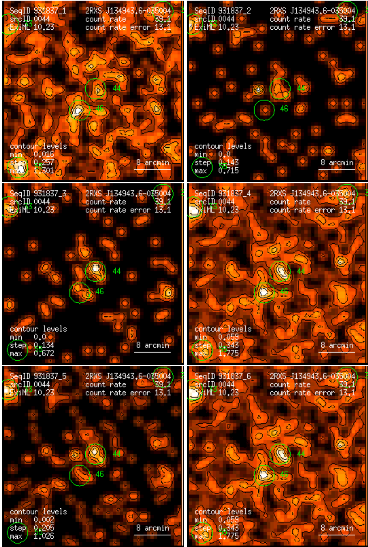
Figure 44: RASS 931837: detection 0044: band rate images, Gaussian filter: (1) PSPC channels 11 – 41, (2) 52 – 90, (3) 91 – 201, (4) 11 – 235, (5) 52 – 201, (6) 11 – 201. Broad band rates in counts/ks. Band rate contour levels in counts/ks/arcmin 2 .
