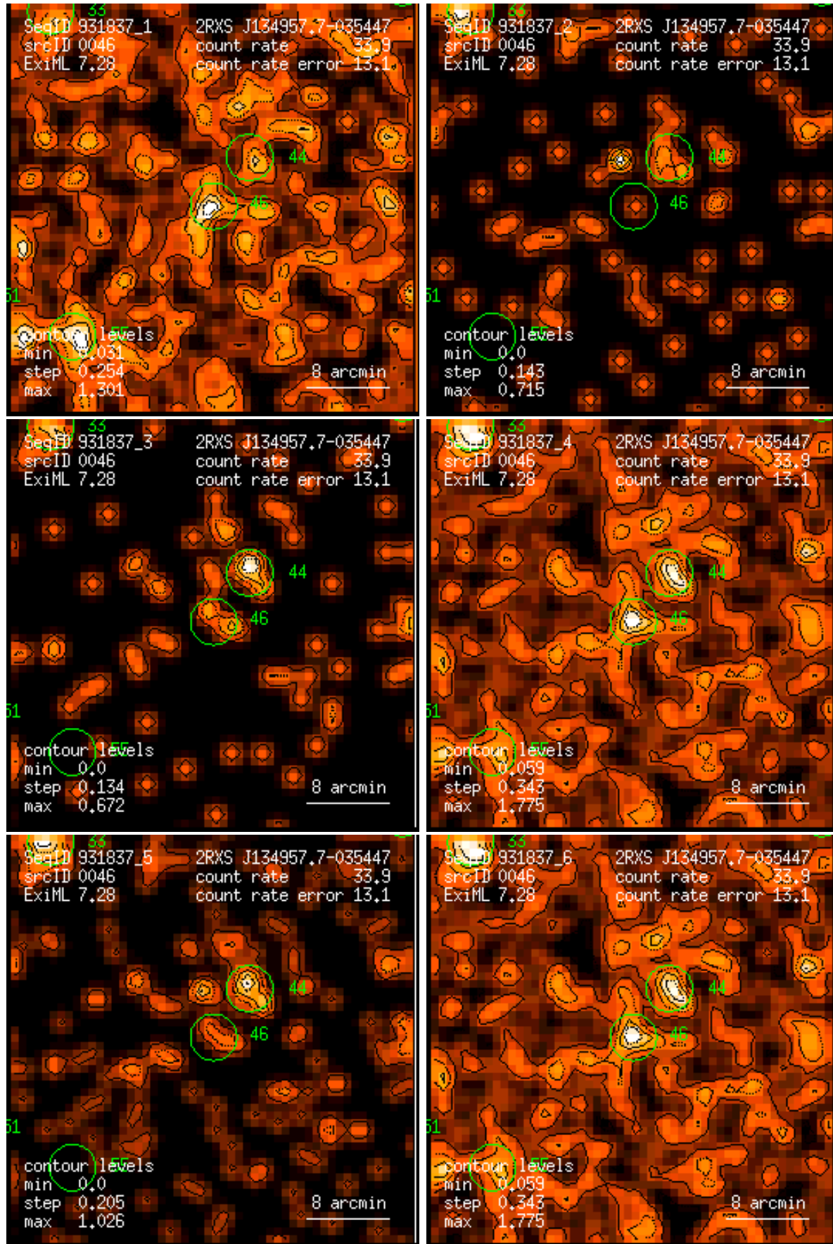
Figure 46: RASS 931837: detection 0046: band rate images, Gaussian filter: (1) PSPC channels 11 – 41, (2) 52 – 90, (3) 91 – 201, (4) 11 – 235, (5) 52 – 201, (6) 11 – 201. Broad band rates in counts/ks. Band rate contour levels in counts/ks/arcmin 2 .
