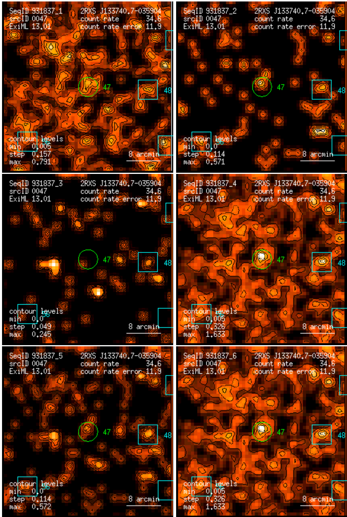
Figure 47: RASS 931837: detection 0047: band rate images, Gaussian filter: (1) PSPC channels 11 – 41, (2) 52 – 90, (3) 91 – 201, (4) 11 – 235, (5) 52 – 201, (6) 11 – 201. Broad band rates in counts/ks. Band rate contour levels in counts/ks/arcmin 2 .
