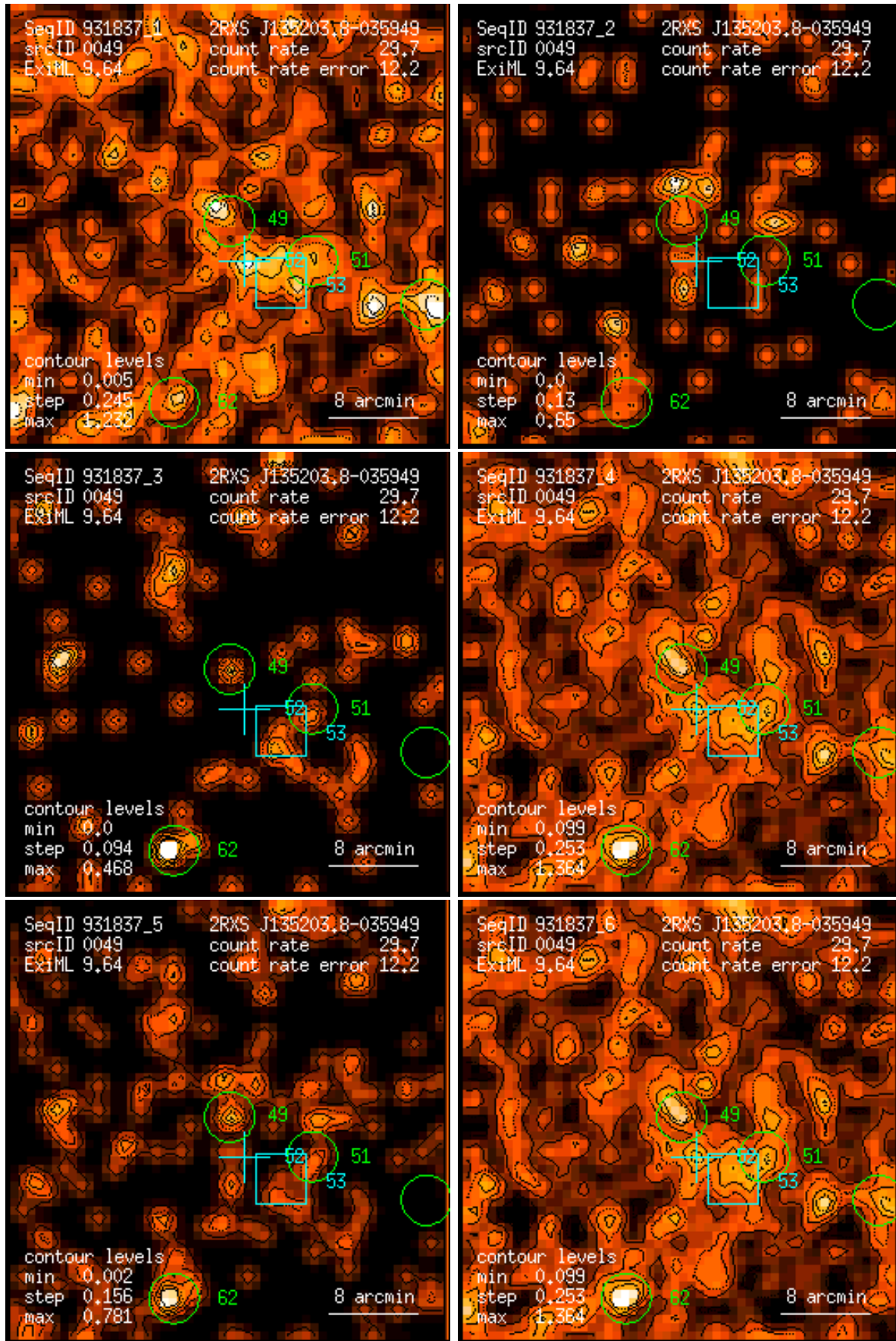
Figure 49: RASS 931837: detection 0049: band rate images, Gaussian filter: (1) PSPC channels 11 – 41, (2) 52 – 90, (3) 91 – 201, (4) 11 – 235, (5) 52 – 201, (6) 11 – 201. Broad band rates in counts/ks. Band rate contour levels in counts/ks/arcmin 2 .
