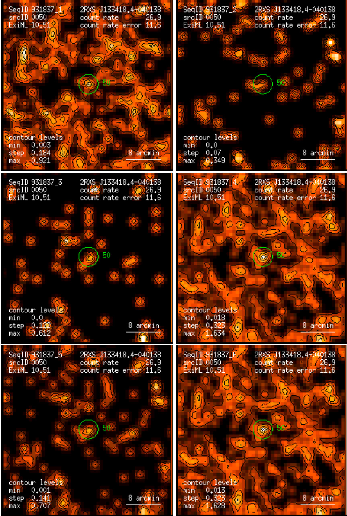
Figure 50: RASS 931837: detection 0050: band rate images, Gaussian filter: (1) PSPC channels 11 – 41, (2) 52 – 90, (3) 91 – 201, (4) 11 – 235, (5) 52 – 201, (6) 11 – 201. Broad band rates in counts/ks. Band rate contour levels in counts/ks/arcmin 2 .
