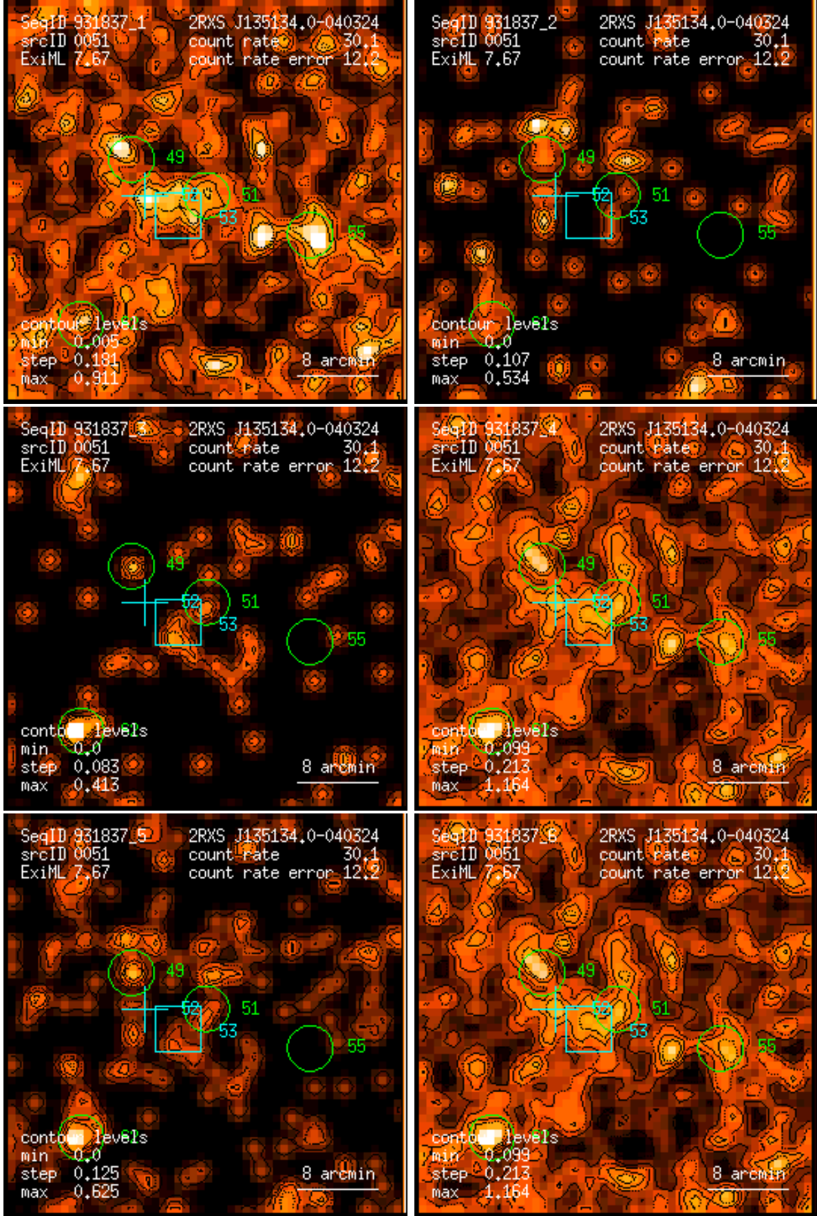
Figure 51: RASS 931837: detection 0051: band rate images, Gaussian filter: (1) PSPC channels 11 – 41, (2) 52 – 90, (3) 91 – 201, (4) 11 – 235, (5) 52 – 201, (6) 11 – 201. Broad band rates in counts/ks. Band rate contour levels in counts/ks/arcmin 2 .
