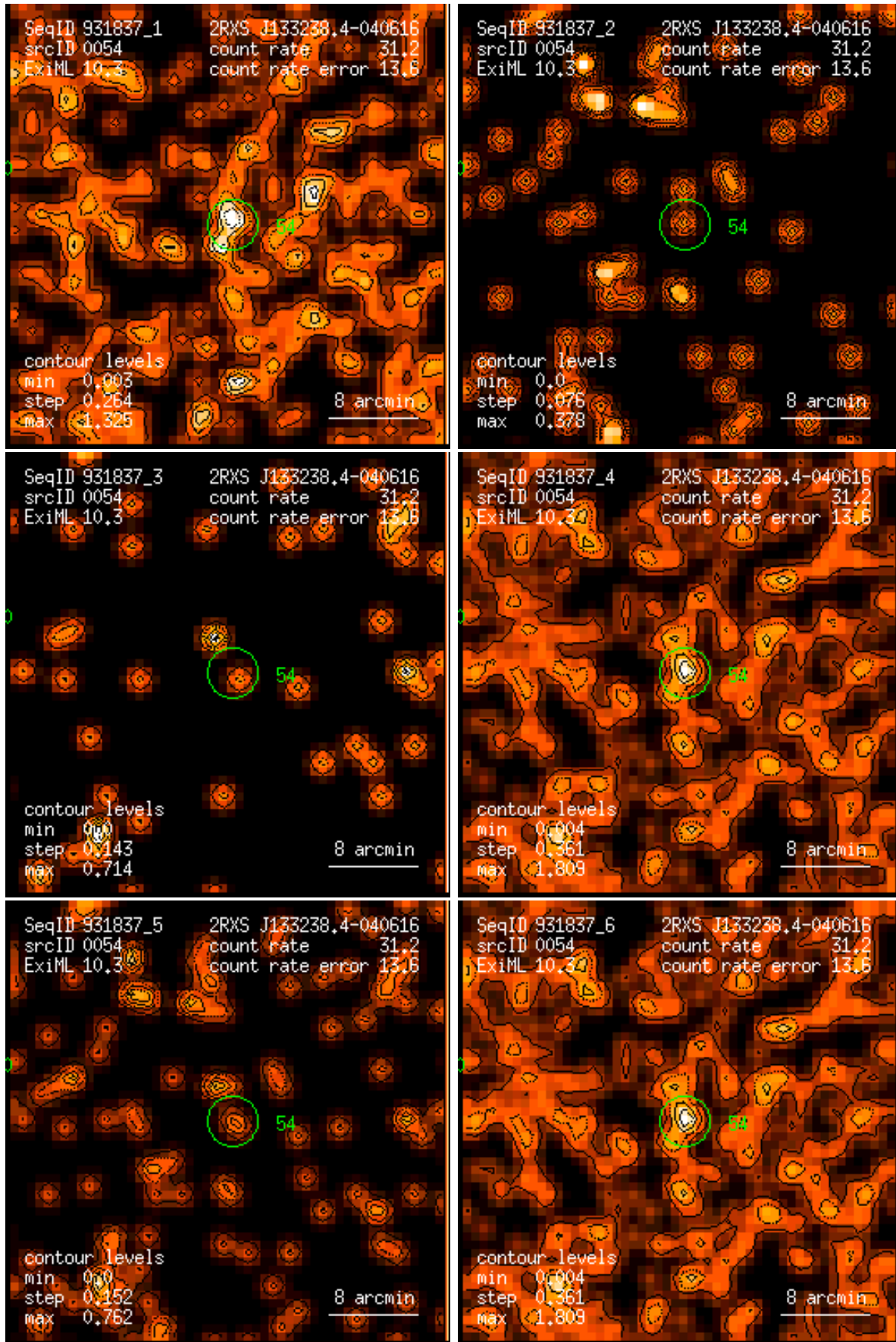
Figure 54: RASS 931837: detection 0054: band rate images, Gaussian filter: (1) PSPC channels 11 – 41, (2) 52 – 90, (3) 91 – 201, (4) 11 – 235, (5) 52 – 201, (6) 11 – 201. Broad band rates in counts/ks. Band rate contour levels in counts/ks/arcmin 2 .
