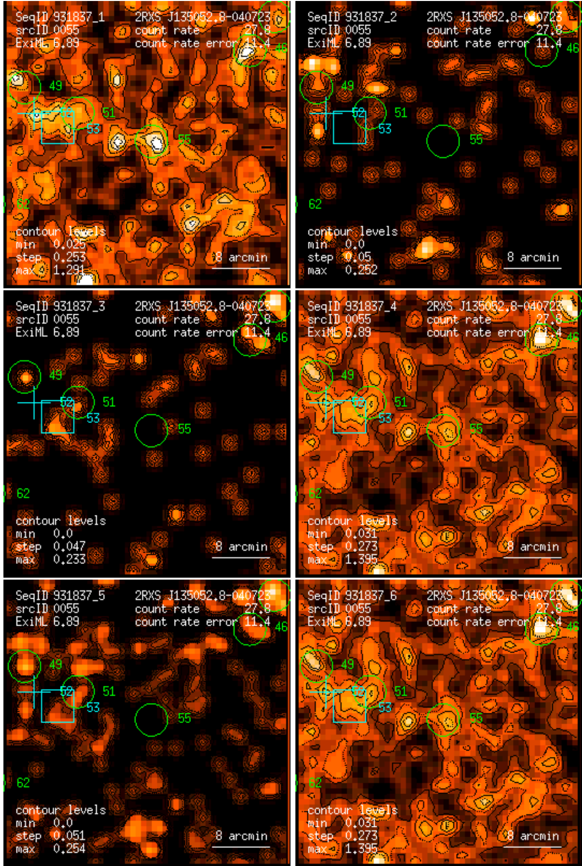
Figure 55: RASS 931837: detection 0055: band rate images, Gaussian filter: (1) PSPC channels 11 – 41, (2) 52 – 90, (3) 91 – 201, (4) 11 – 235, (5) 52 – 201, (6) 11 – 201. Broad band rates in counts/ks. Band rate contour levels in counts/ks/arcmin 2 .
