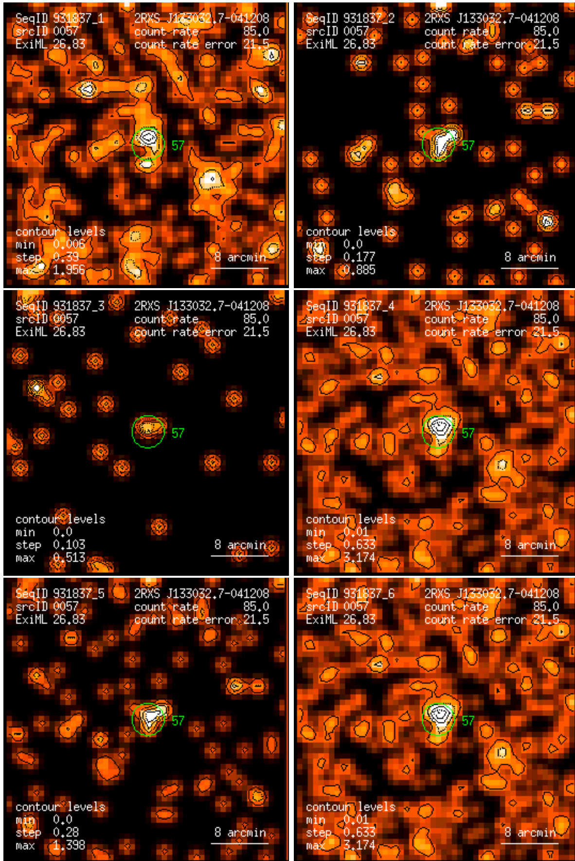
Figure 57: RASS 931837: detection 0057: band rate images, Gaussian filter: (1) PSPC channels 11 – 41, (2) 52 – 90, (3) 91 – 201, (4) 11 – 235, (5) 52 – 201, (6) 11 – 201. Broad band rates in counts/ks. Band rate contour levels in counts/ks/arcmin 2 .
