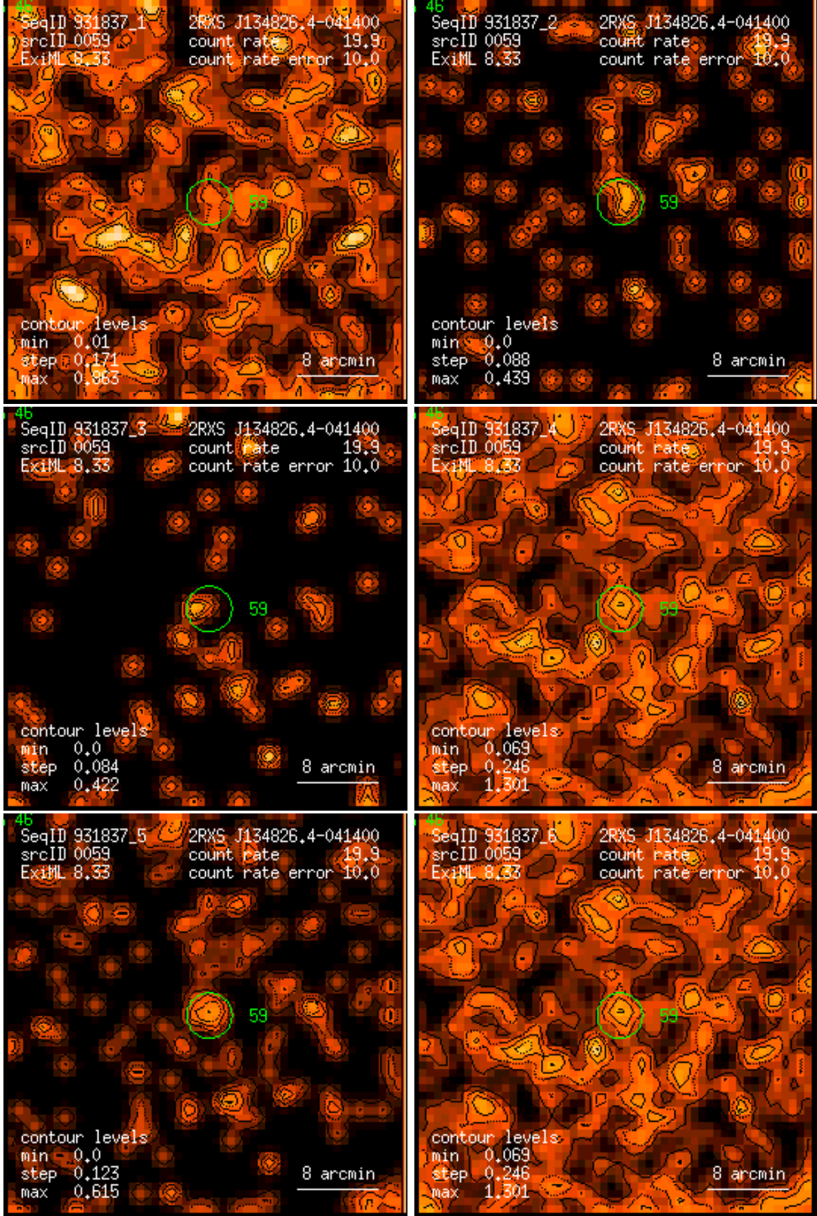
Figure 59: RASS 931837: detection 0059: band rate images, Gaussian filter: (1) PSPC channels 11 – 41, (2) 52 – 90, (3) 91 – 201, (4) 11 – 235, (5) 52 – 201, (6) 11 – 201. Broad band rates in counts/ks. Band rate contour levels in counts/ks/arcmin 2 .
