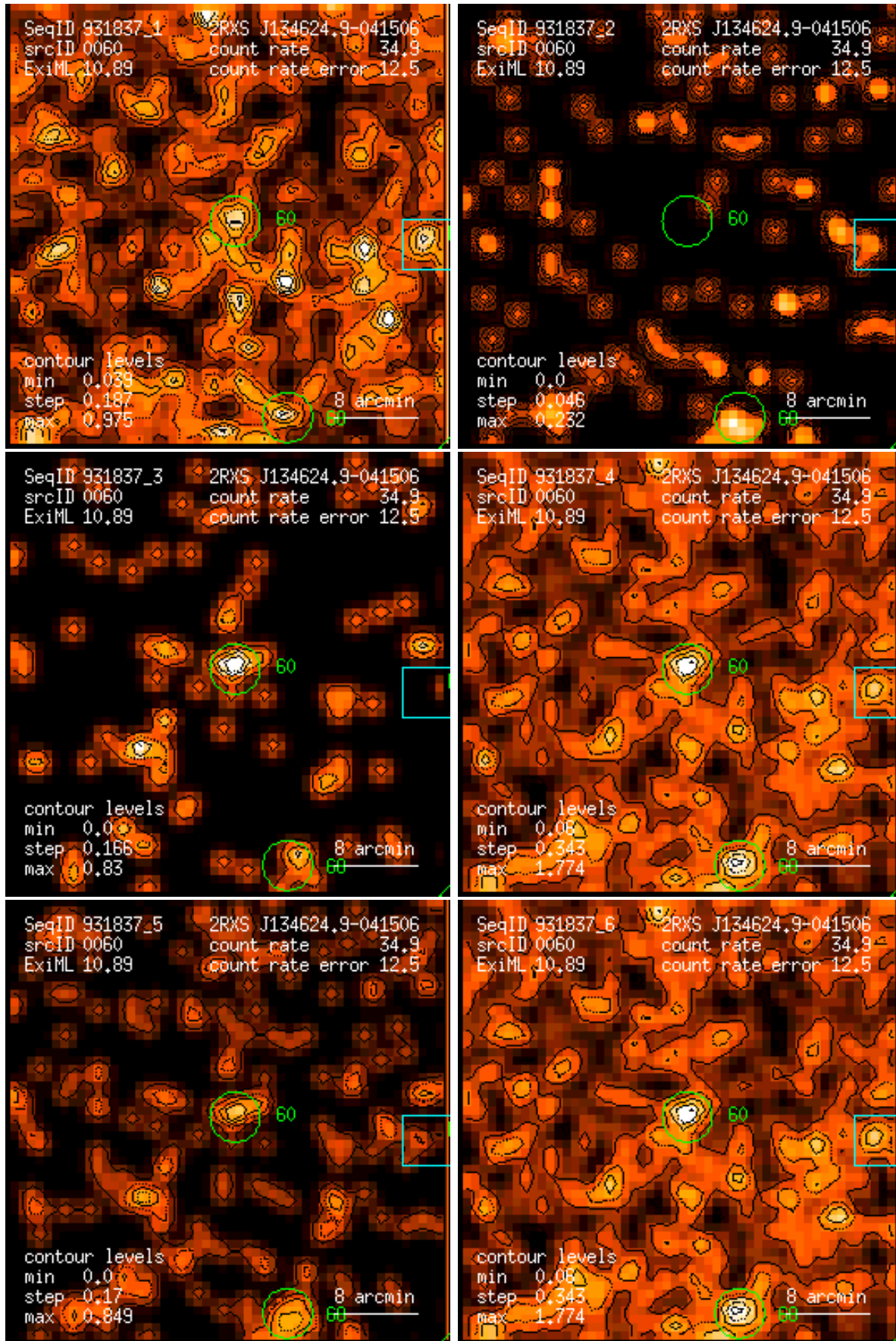
Figure 60: RASS 931837: detection 0060: band rate images, Gaussian filter: (1) PSPC channels 11 – 41, (2) 52 – 90, (3) 91 – 201, (4) 11 – 235, (5) 52 – 201, (6) 11 – 201. Broad band rates in counts/ks. Band rate contour levels in counts/ks/arcmin 2 .
