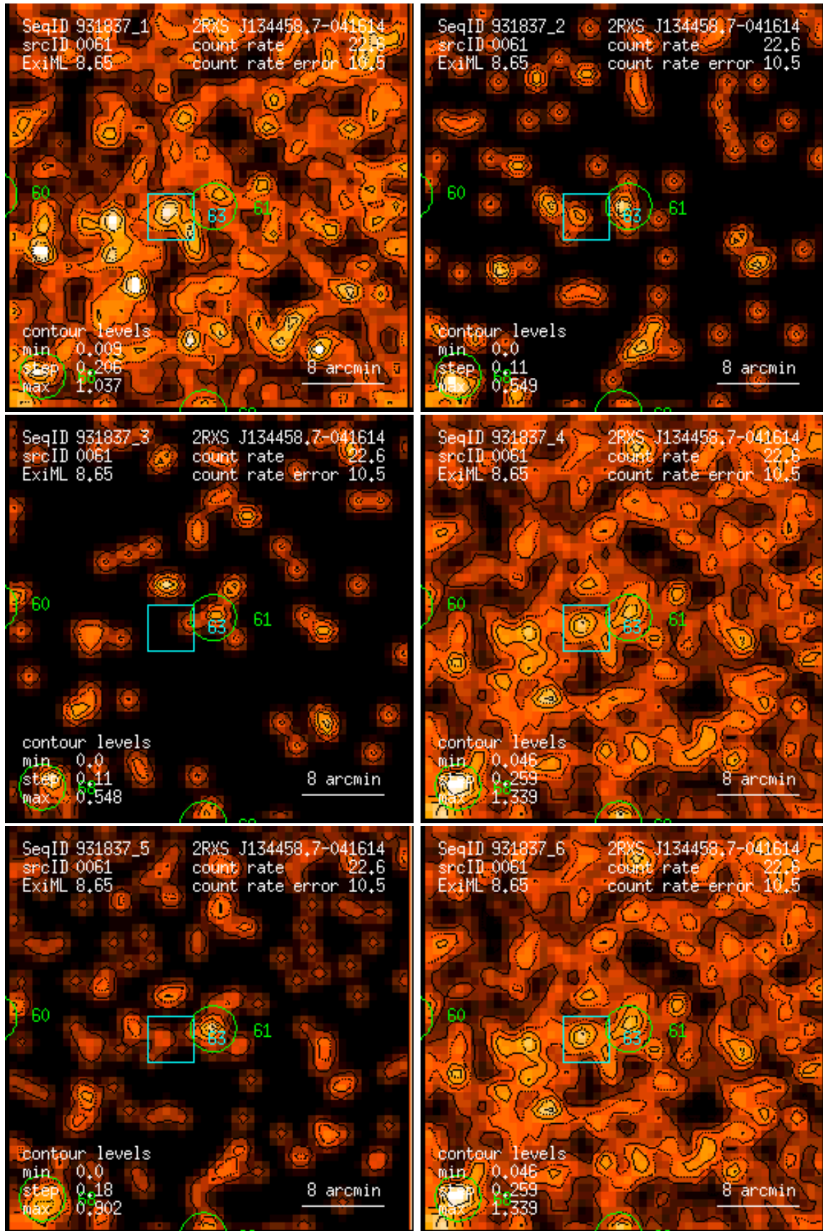
Figure 61: RASS 931837: detection 0061: band rate images, Gaussian filter: (1) PSPC channels 11 – 41, (2) 52 – 90, (3) 91 – 201, (4) 11 – 235, (5) 52 – 201, (6) 11 – 201. Broad band rates in counts/ks. Band rate contour levels in counts/ks/arcmin 2 .
