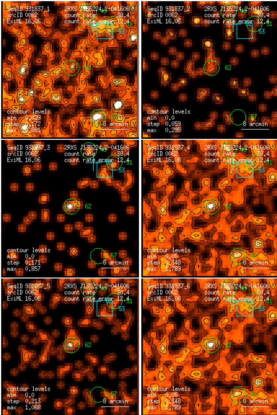
Figure 62: RASS 931837: detection 0062: band rate images, Gaussian filter: (1) PSPC channels 11 – 41, (2) 52 – 90, (3) 91 – 201, (4) 11 – 235, (5) 52 – 201, (6) 11 – 201. Broad band rates in counts/ks. Band rate contour levels in counts/ks/arcmin 2 .
