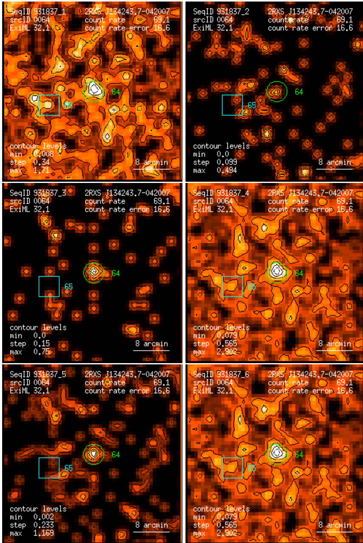
Figure 64: RASS 931837: detection 0064: band rate images, Gaussian filter: (1) PSPC channels 11 – 41, (2) 52 – 90, (3) 91 – 201, (4) 11 – 235, (5) 52 – 201, (6) 11 – 201. Broad band rates in counts/ks. Band rate contour levels in counts/ks/arcmin 2 .
