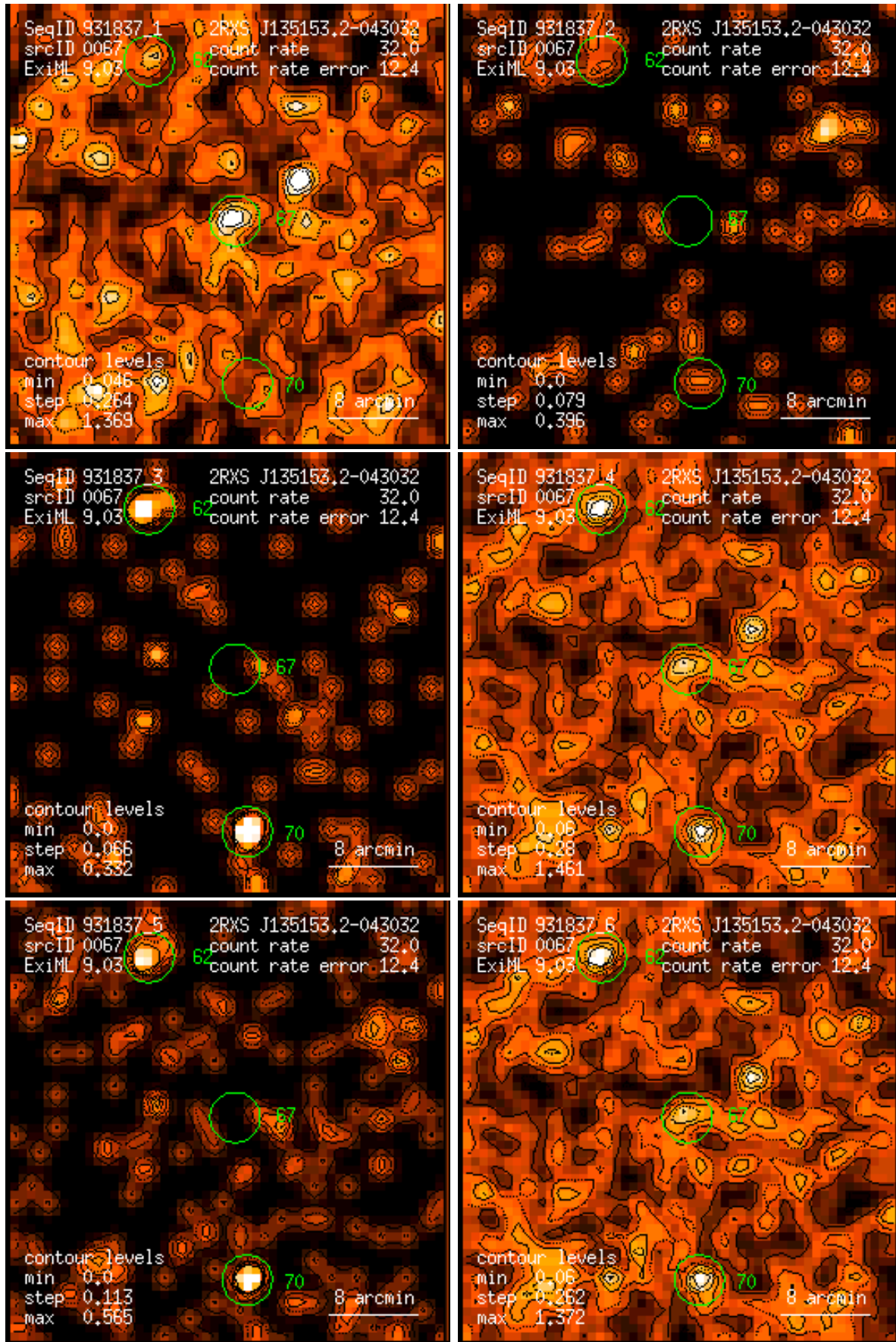
Figure 67: RASS 931837: detection 0067: band rate images, Gaussian filter: (1) PSPC channels 11 – 41, (2) 52 – 90, (3) 91 – 201, (4) 11 – 235, (5) 52 – 201, (6) 11 – 201. Broad band rates in counts/ks. Band rate contour levels in counts/ks/arcmin 2 .
