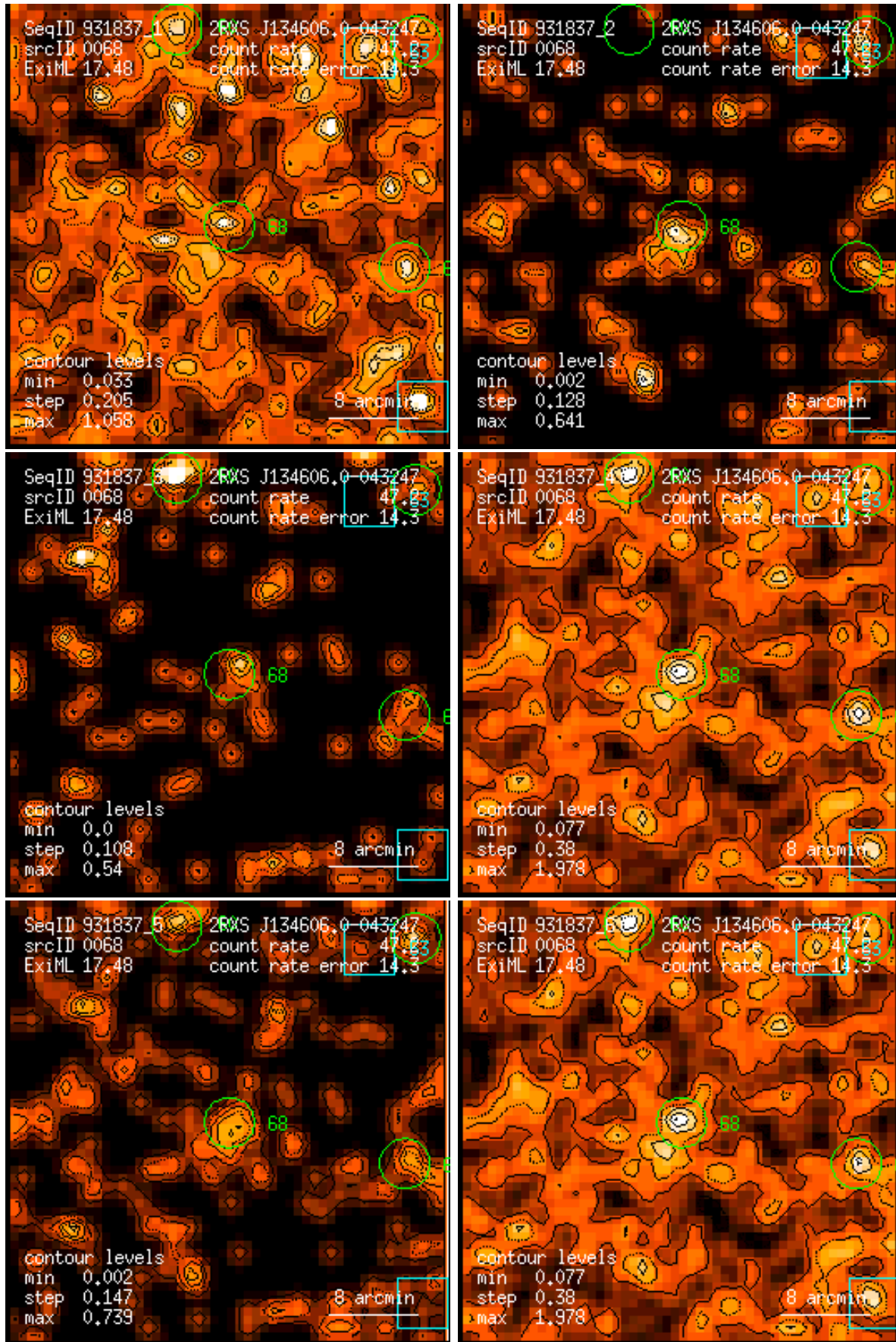
Figure 68: RASS 931837: detection 0068: band rate images, Gaussian filter: (1) PSPC channels 11 – 41, (2) 52 – 90, (3) 91 – 201, (4) 11 – 235, (5) 52 – 201, (6) 11 – 201. Broad band rates in counts/ks. Band rate contour levels in counts/ks/arcmin 2 .
