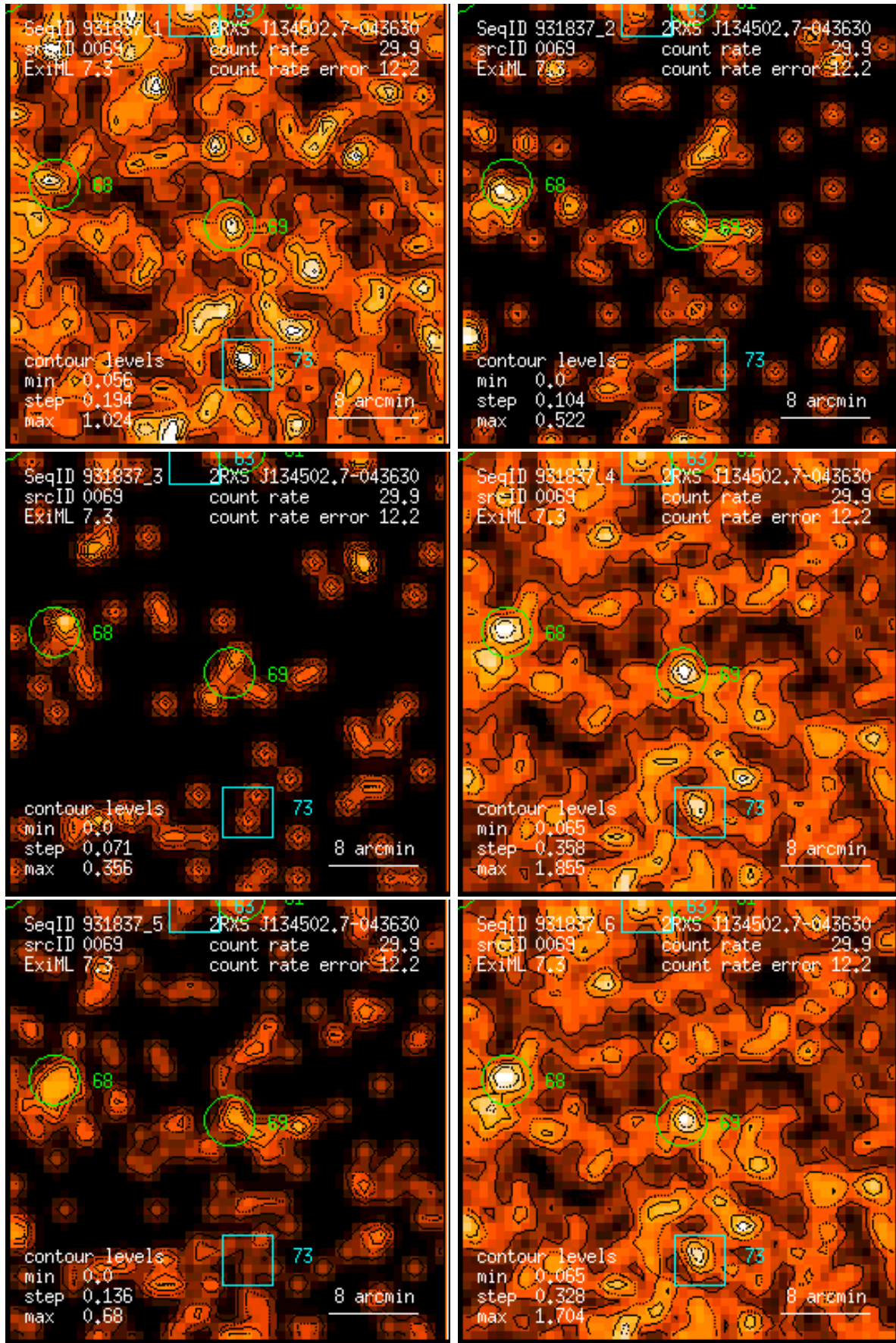
Figure 69: RASS 931837: detection 0069: band rate images, Gaussian filter: (1) PSPC channels 11 – 41, (2) 52 – 90, (3) 91 – 201, (4) 11 – 235, (5) 52 – 201, (6) 11 – 201. Broad band rates in counts/ks. Band rate contour levels in counts/ks/arcmin 2 .
