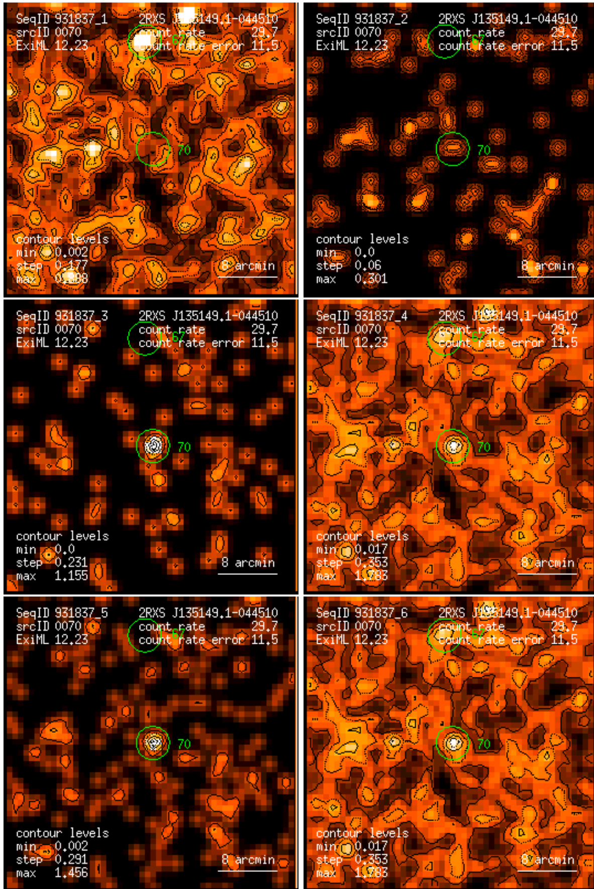
Figure 70: RASS 931837: detection 0070: band rate images, Gaussian filter: (1) PSPC channels 11 – 41, (2) 52 – 90, (3) 91 – 201, (4) 11 – 235, (5) 52 – 201, (6) 11 – 201. Broad band rates in counts/ks. Band rate contour levels in counts/ks/arcmin 2 .
