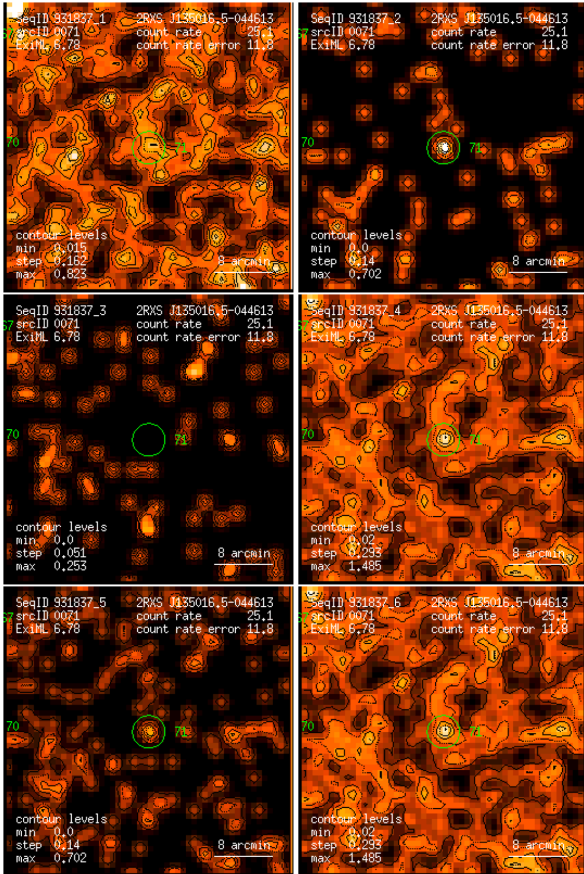
Figure 71: RASS 931837: detection 0071: band rate images, Gaussian filter: (1) PSPC channels 11 – 41, (2) 52 – 90, (3) 91 – 201, (4) 11 – 235, (5) 52 – 201, (6) 11 – 201. Broad band rates in counts/ks. Band rate contour levels in counts/ks/arcmin 2 .
