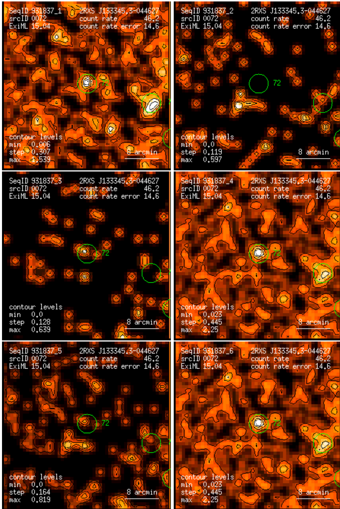
Figure 72: RASS 931837: detection 0072: band rate images, Gaussian filter: (1) PSPC channels 11 – 41, (2) 52 – 90, (3) 91 – 201, (4) 11 – 235, (5) 52 – 201, (6) 11 – 201. Broad band rates in counts/ks. Band rate contour levels in counts/ks/arcmin 2 .
