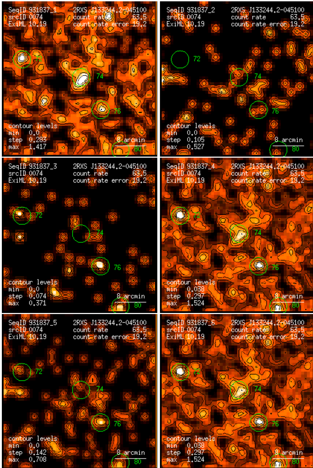
Figure 74: RASS 931837: detection 0074: band rate images, Gaussian filter: (1) PSPC channels 11 – 41, (2) 52 – 90, (3) 91 – 201, (4) 11 – 235, (5) 52 – 201, (6) 11 – 201. Broad band rates in counts/ks. Band rate contour levels in counts/ks/arcmin 2 .
