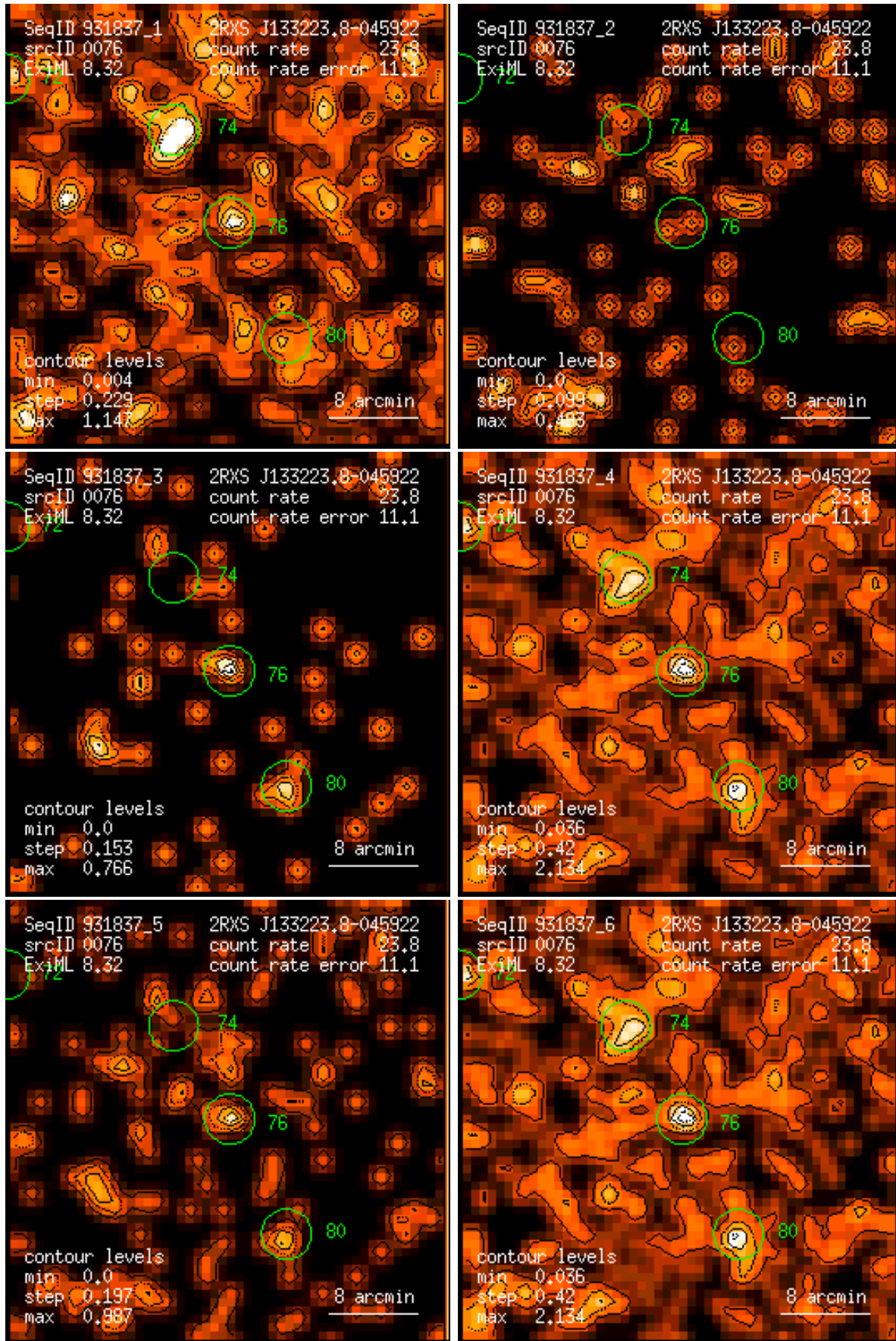
Figure 76: RASS 931837: detection 0076: band rate images, Gaussian filter: (1) PSPC channels 11 – 41, (2) 52 – 90, (3) 91 – 201, (4) 11 – 235, (5) 52 – 201, (6) 11 – 201. Broad band rates in counts/ks. Band rate contour levels in counts/ks/arcmin 2 .
