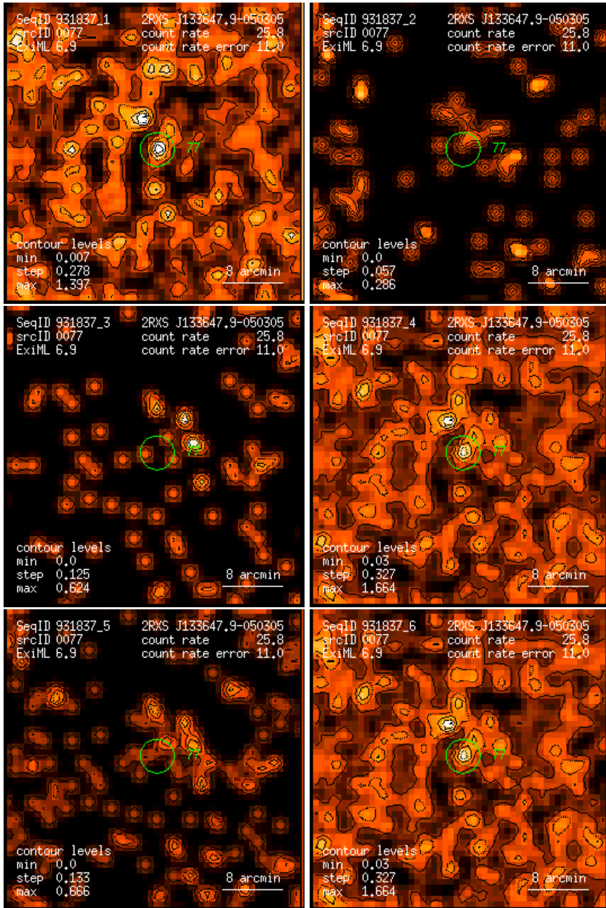
Figure 77: RASS 931837: detection 0077: band rate images, Gaussian filter: (1) PSPC channels 11 – 41, (2) 52 – 90, (3) 91 – 201, (4) 11 – 235, (5) 52 – 201, (6) 11 – 201. Broad band rates in counts/ks. Band rate contour levels in counts/ks/arcmin 2 .
