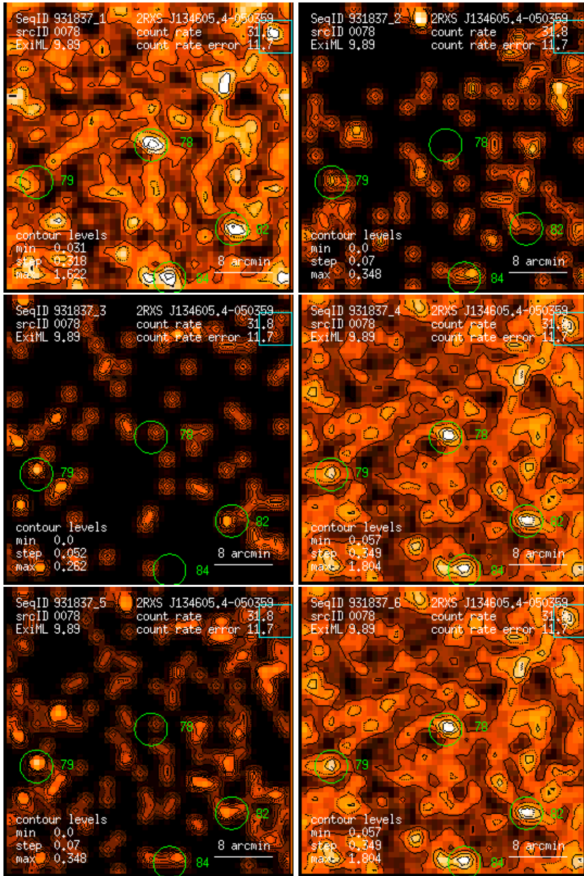
Figure 78: RASS 931837: detection 0078: band rate images, Gaussian filter: (1) PSPC channels 11 – 41, (2) 52 – 90, (3) 91 – 201, (4) 11 – 235, (5) 52 – 201, (6) 11 – 201. Broad band rates in counts/ks. Band rate contour levels in counts/ks/arcmin 2 .
